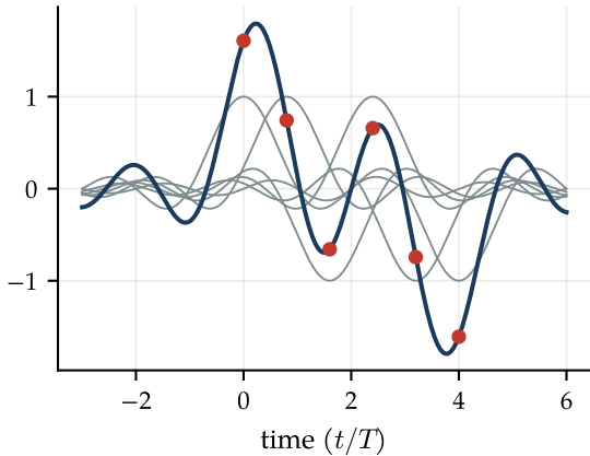
Sinc pulses sent every 0.8T
