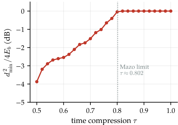
Minimum distance (error events \leq 8 bits)
