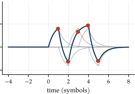
rectangular pulses through an RC low-pass
