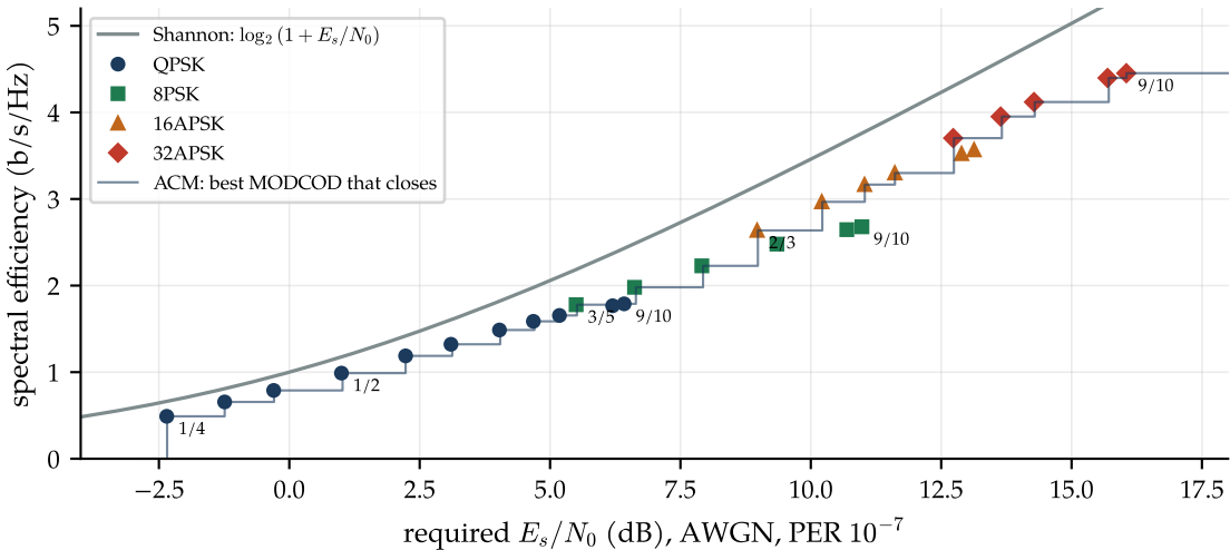
DVB-S2 MODCODs (after ETSI EN 302 307-1)
