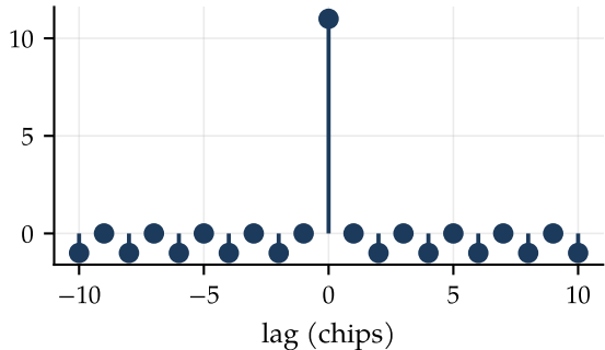
Autocorrelation: peak 11, sidelobes \leq 1
