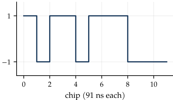
The 11-chip Barker sequence
