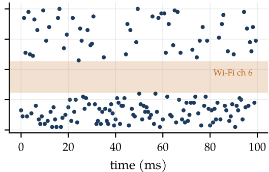
Adaptive frequency hopping: bad channels remapped
