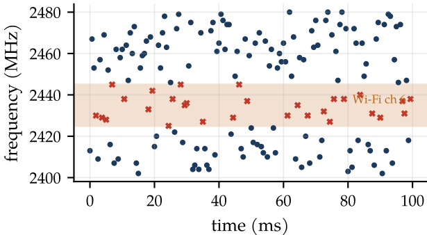
Classic hopping: about one hop in five lands on a busy Wi-Fi channel
