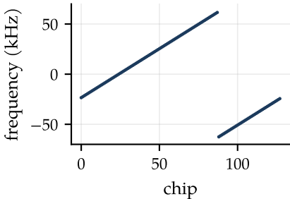
received chirp ( s = 40 )
