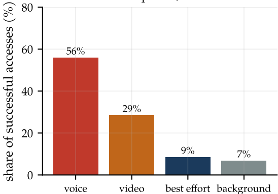
Four saturated queues, EDCA defaults
