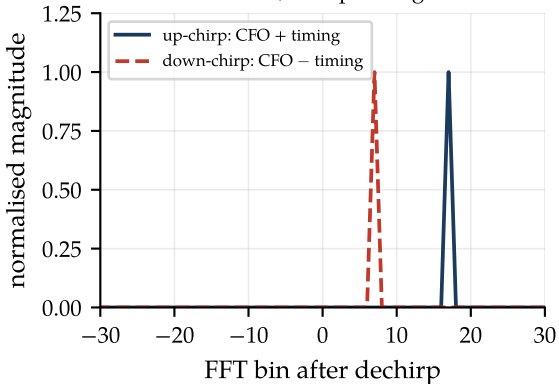
12-bin CFO, 5-chip timing error
