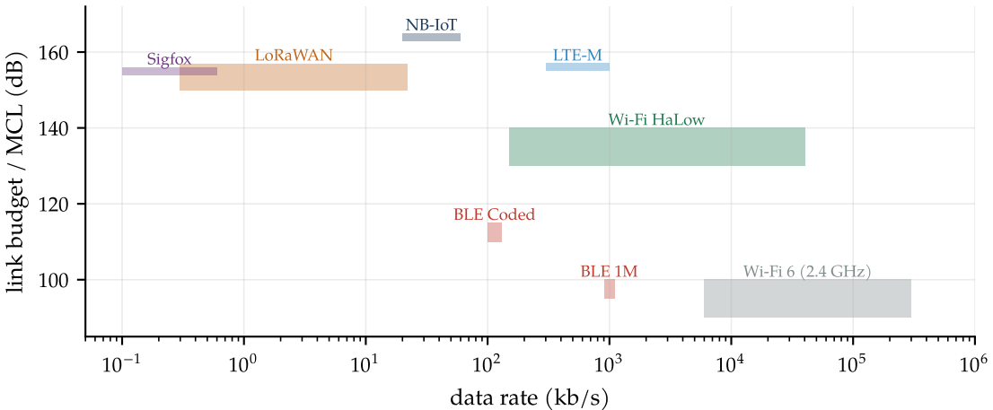
The low-power wide-area trade: every decade of rate costs about 10 dB of reach
