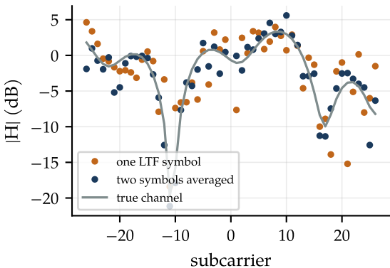
Channel estimate from the L-LTF, 10 dB SNR
