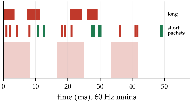
Packets in the oven's off half-cycles survive
