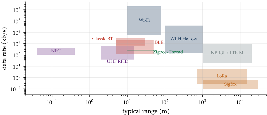
The family portrait: every radio in this chapter (rough, typical values)
