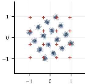
after CMA \rightarrow DD-LMS
