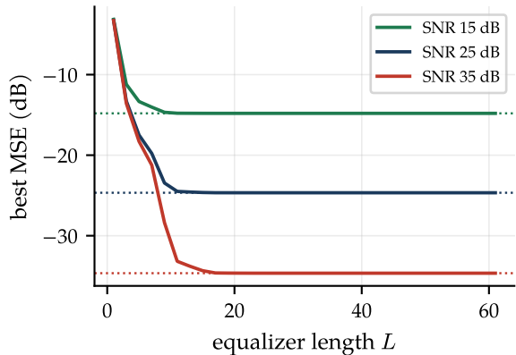
MSE vs. length (dotted: L \rightarrow \infty )
