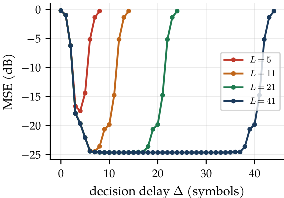
MMSE FIR vs. delay (SNR 25 dB)
