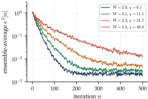
LMS, \mu = 0.05
