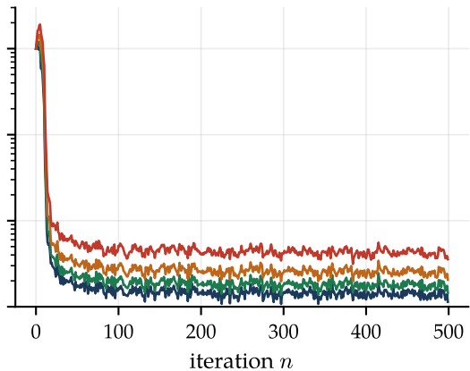
RLS, \lambda = 1, \delta = 0.004
