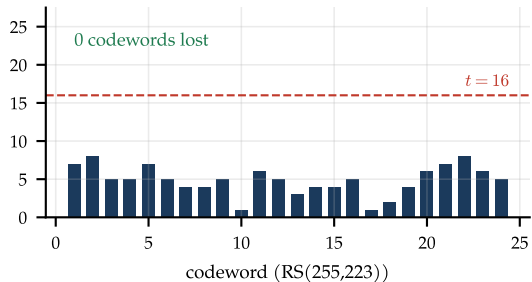
interleaved to depth 24
