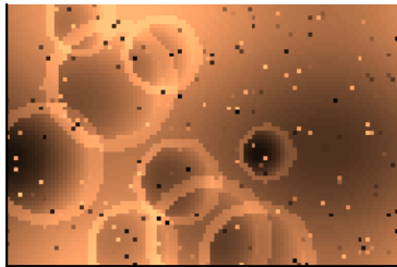
RM(1,5): 3.21% wrong
