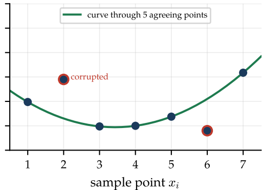
Find the curve most points agree on
