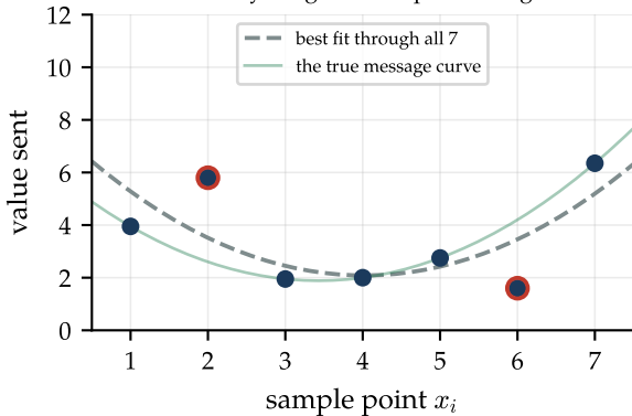
Fit everything: the bad points drag it
