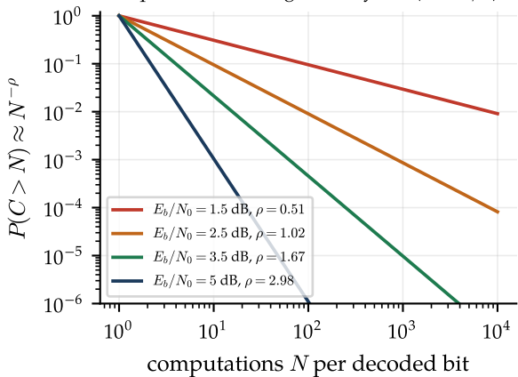
Sequential decoding: a heavy tail ( R = 1/2 )
