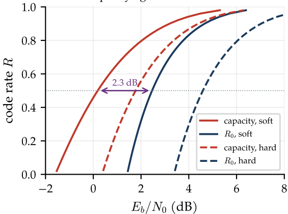
Capacity against the cutoff rate
