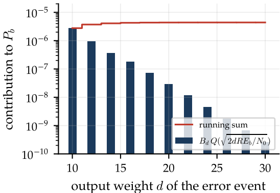
K = 7 union bound at 4.4 dB
