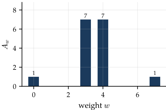
Hamming (7,4): 16 codewords
