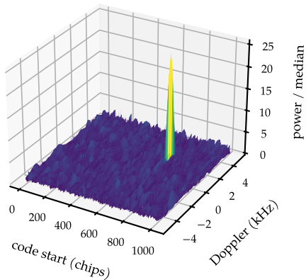
(a) PRN 7, 44 dB-Hz, 4 \times 1 ms
