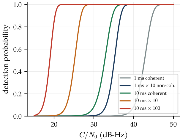
(b) P_{fa} = 10^{-6} per cell, 1.5 dB loss
