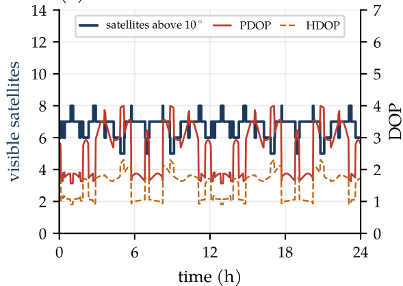
(b) 24-satellite Walker model
