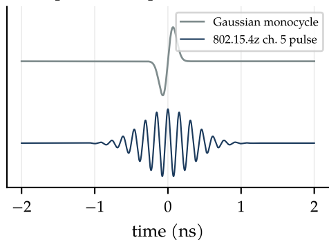
(c) impulse-radio pulses
