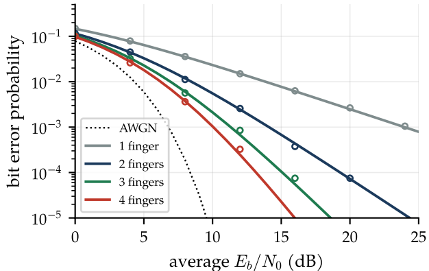
(b) Rayleigh paths, MRC Rake
