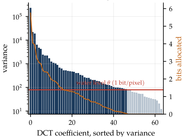
Portrait, 8×8 DCT: gain 12.6 dB
