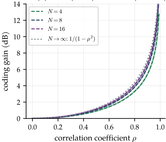
AR(1): KLT (solid) and DCT (dashed)
