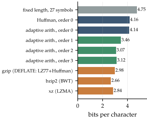
Compressing 34k characters
