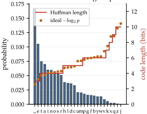
Letter statistics of English prose
