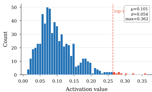
(a) Neuron #20 activation distribution
