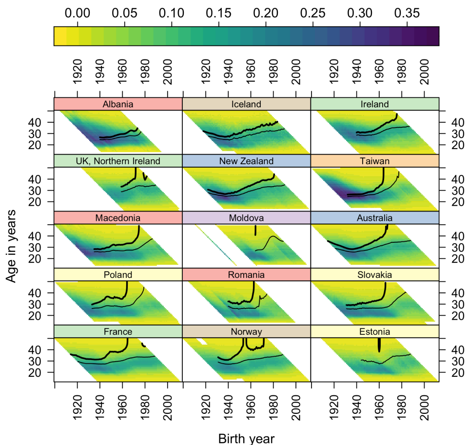
Figure 2: The fifteen highest-ranked countries by CPCFR at 2007, updated to 2023–25.
