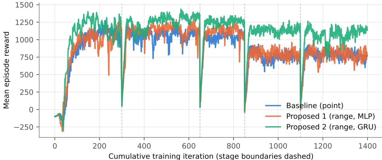
Training reward across the 5-stage curriculum (seed 42)
