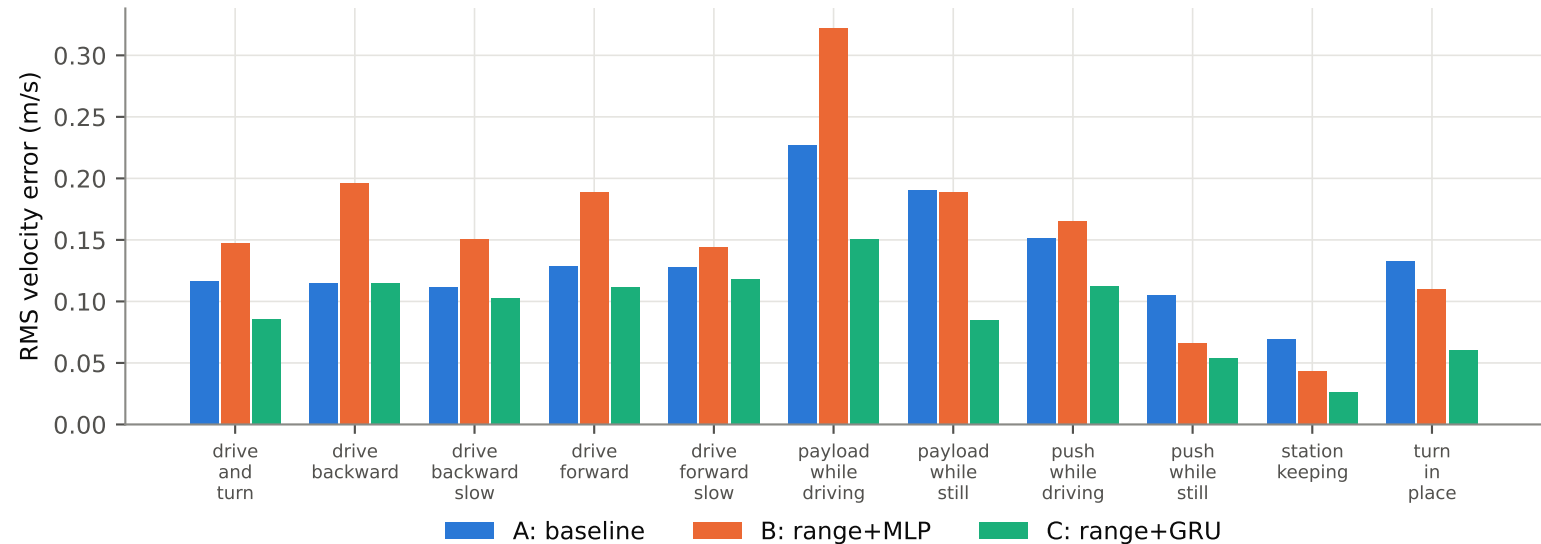
Velocity-tracking error by scenario, all three arms under measured-range DR
