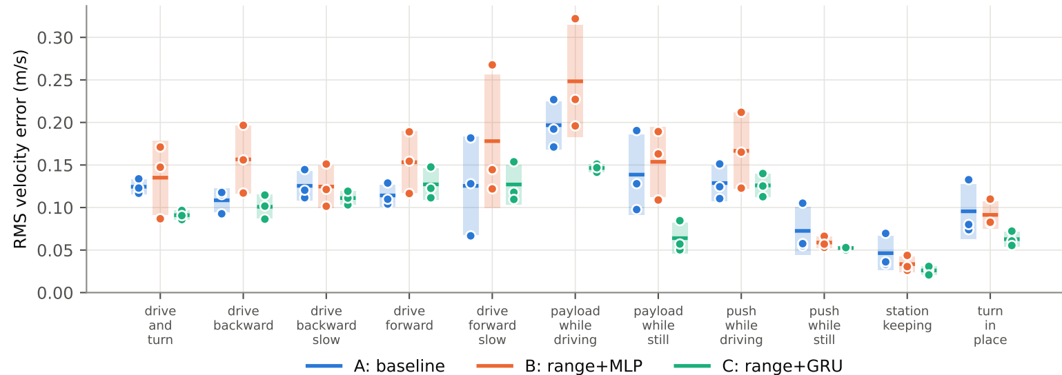
Velocity-tracking error by scenario, all three arms under measured-range DR (mean \pm s.d. over 3 seeds)
