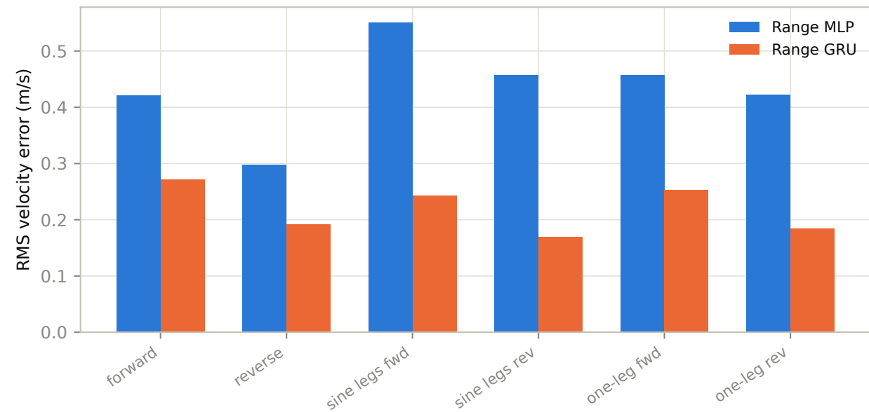
Command-tracking error comparison
