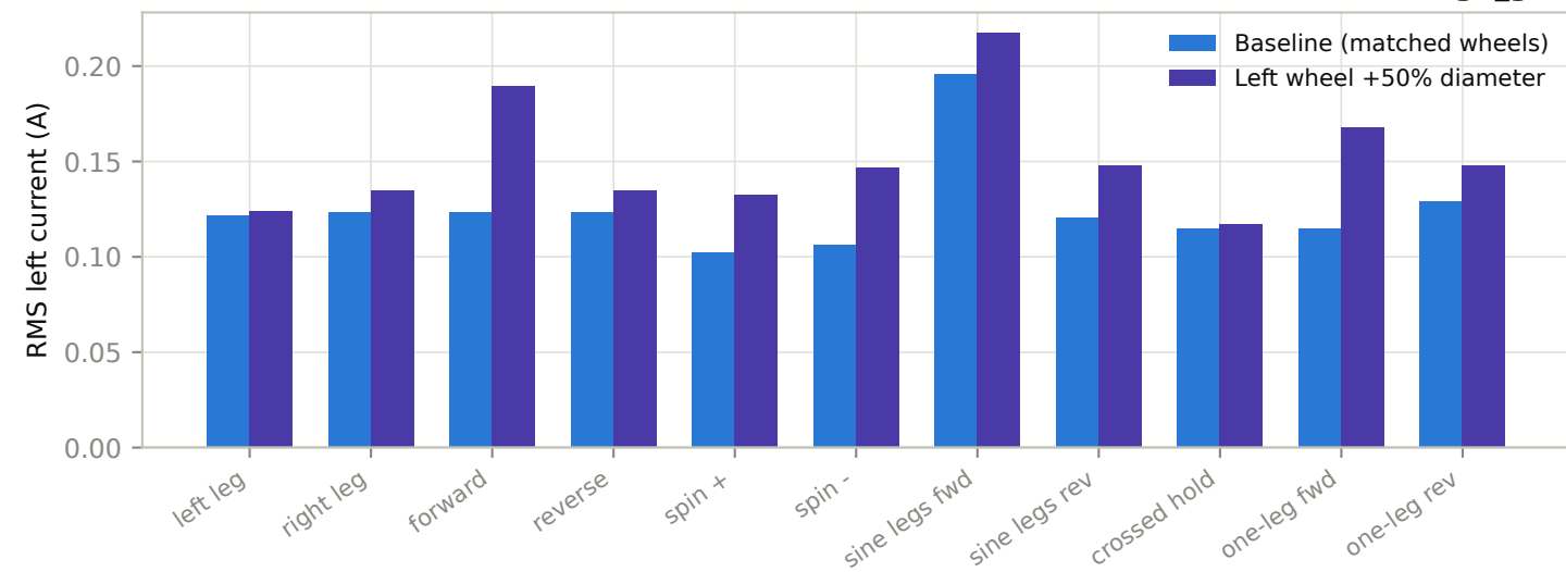
Per-wheel DDSM115 current: matched wheels vs. left wheel +50% diameter (range_gru)
