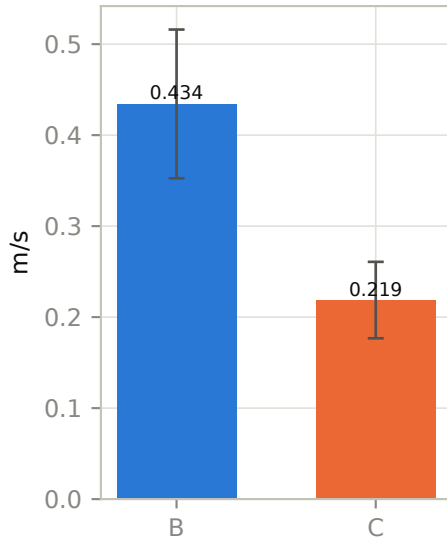
RMS velocity error (n=6 stages)
