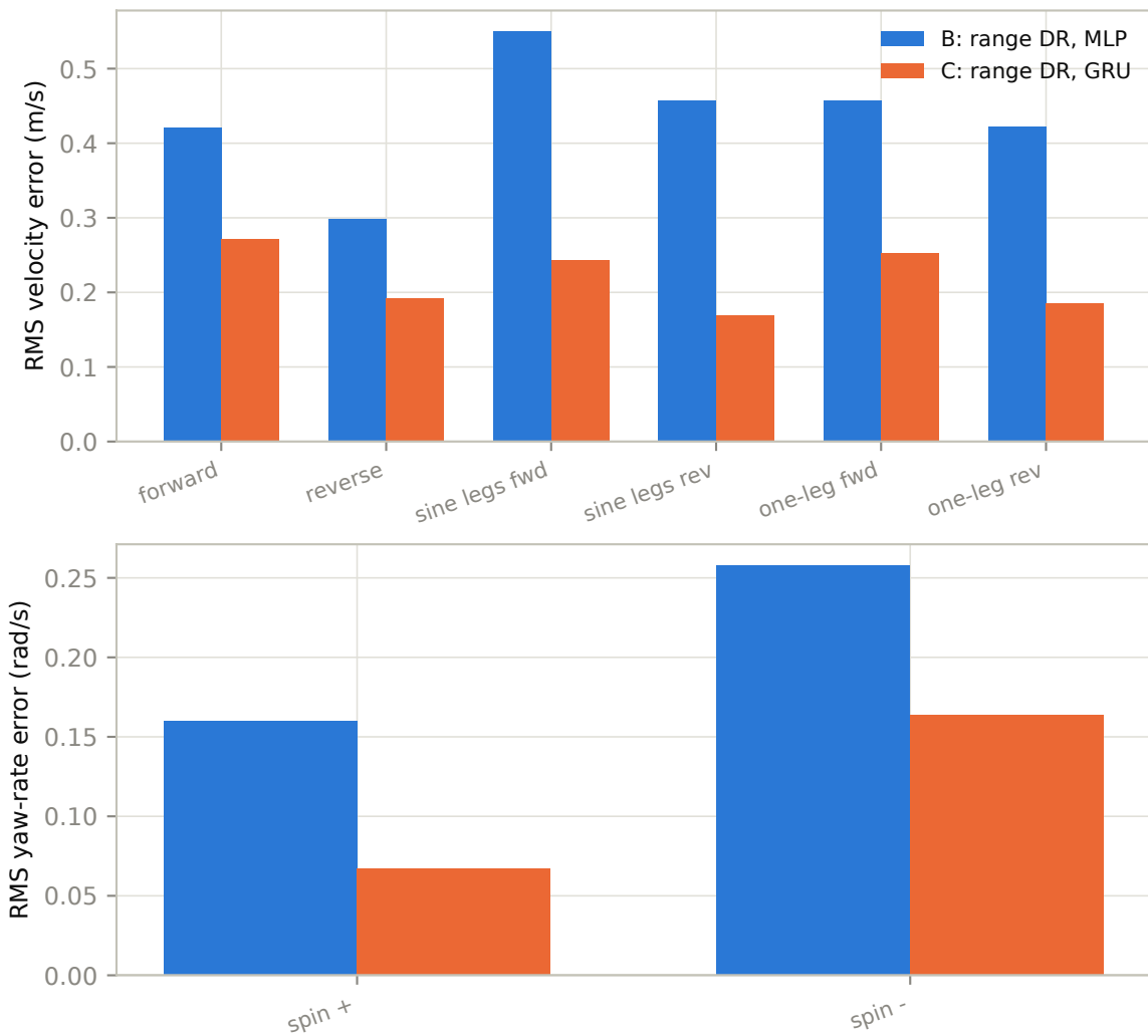
Hardware command-tracking error by test-bench scenario
