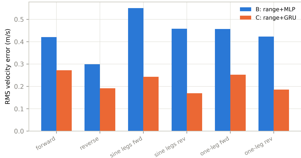
Scenario-wise RMS longitudinal-velocity tracking error, hardware (B vs C)
