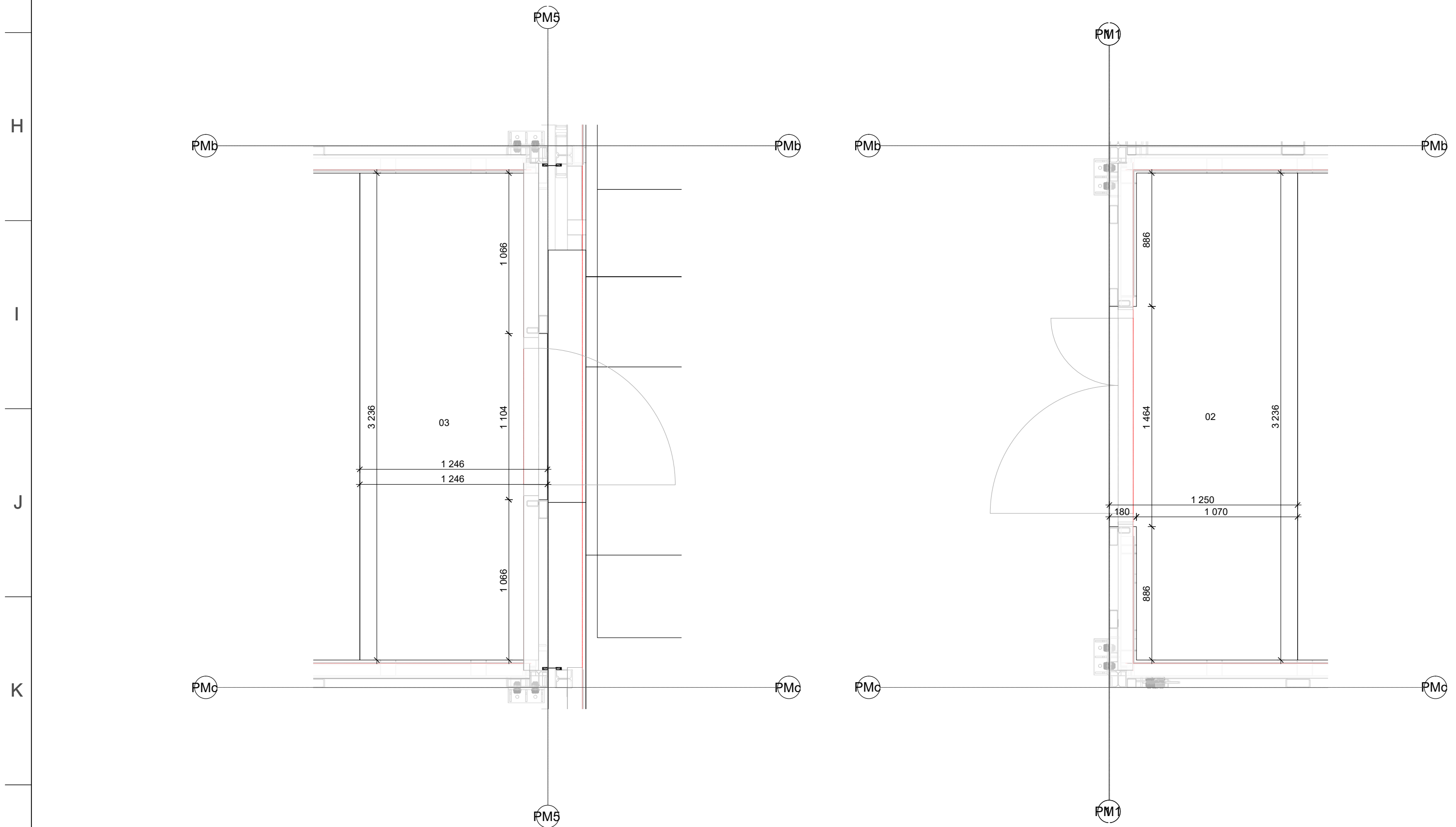
03 PM - Floor Plan - Cement Fibre - Board pos. 03 1 : 25
