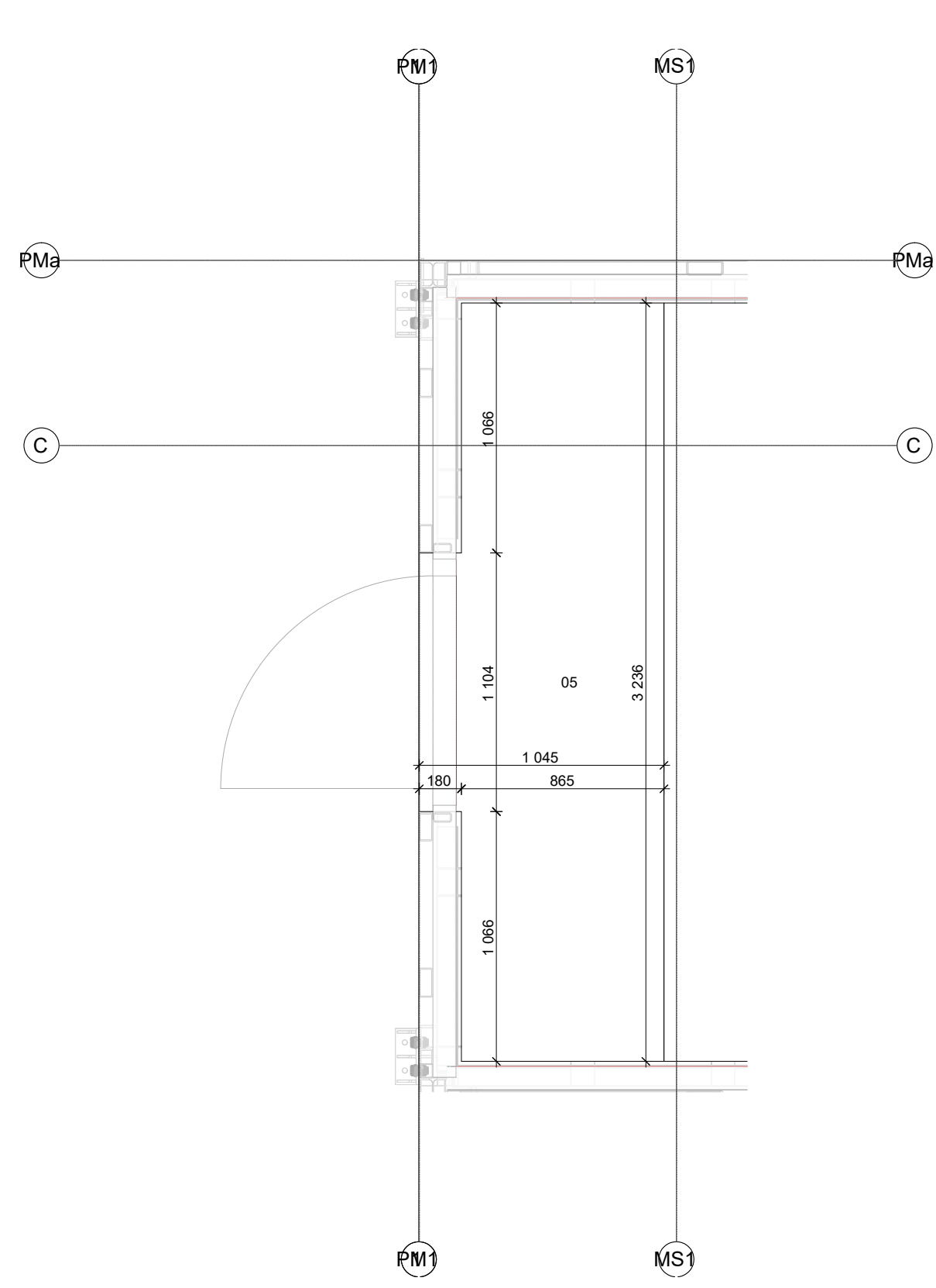
05 PM - Floor Plan - Cement Fibre - Board pos. 05 1 : 25
