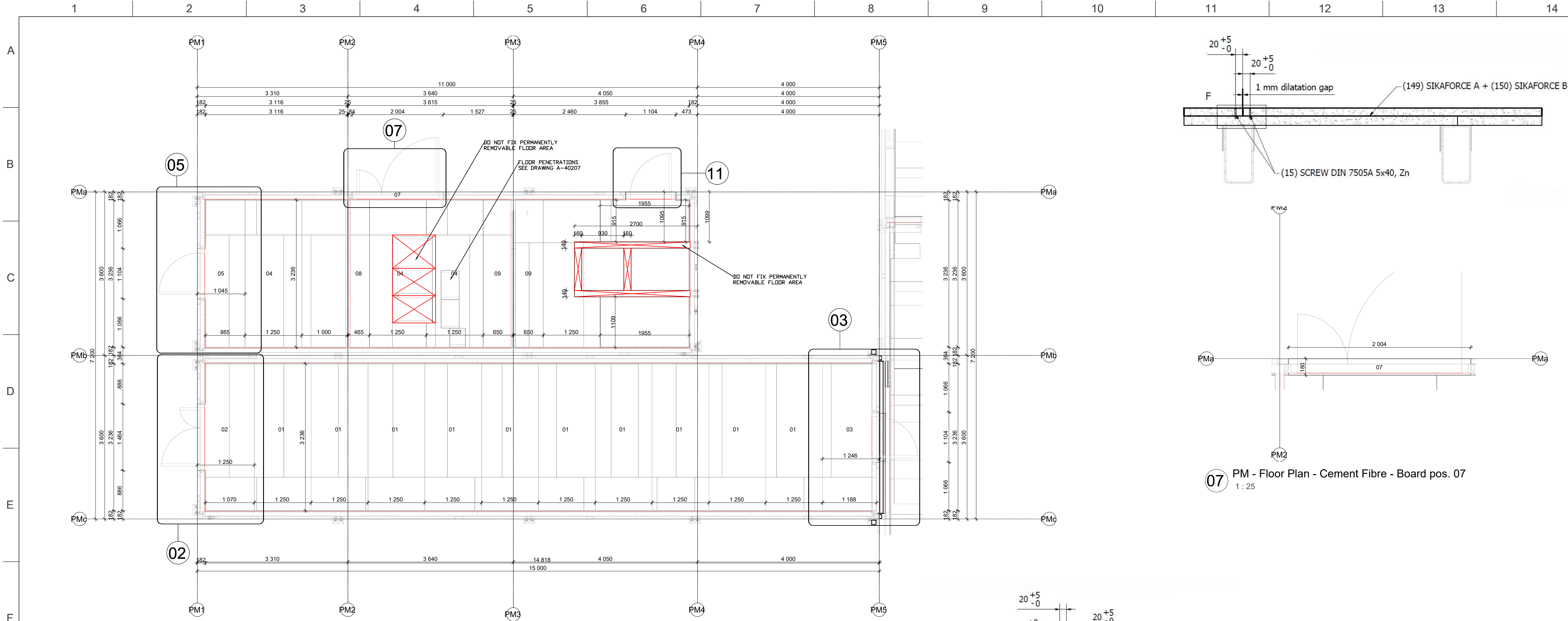
1 PM - FIRST FLOOR LAYER LAYOUT - CEMENT FIBRE 1 : 50
