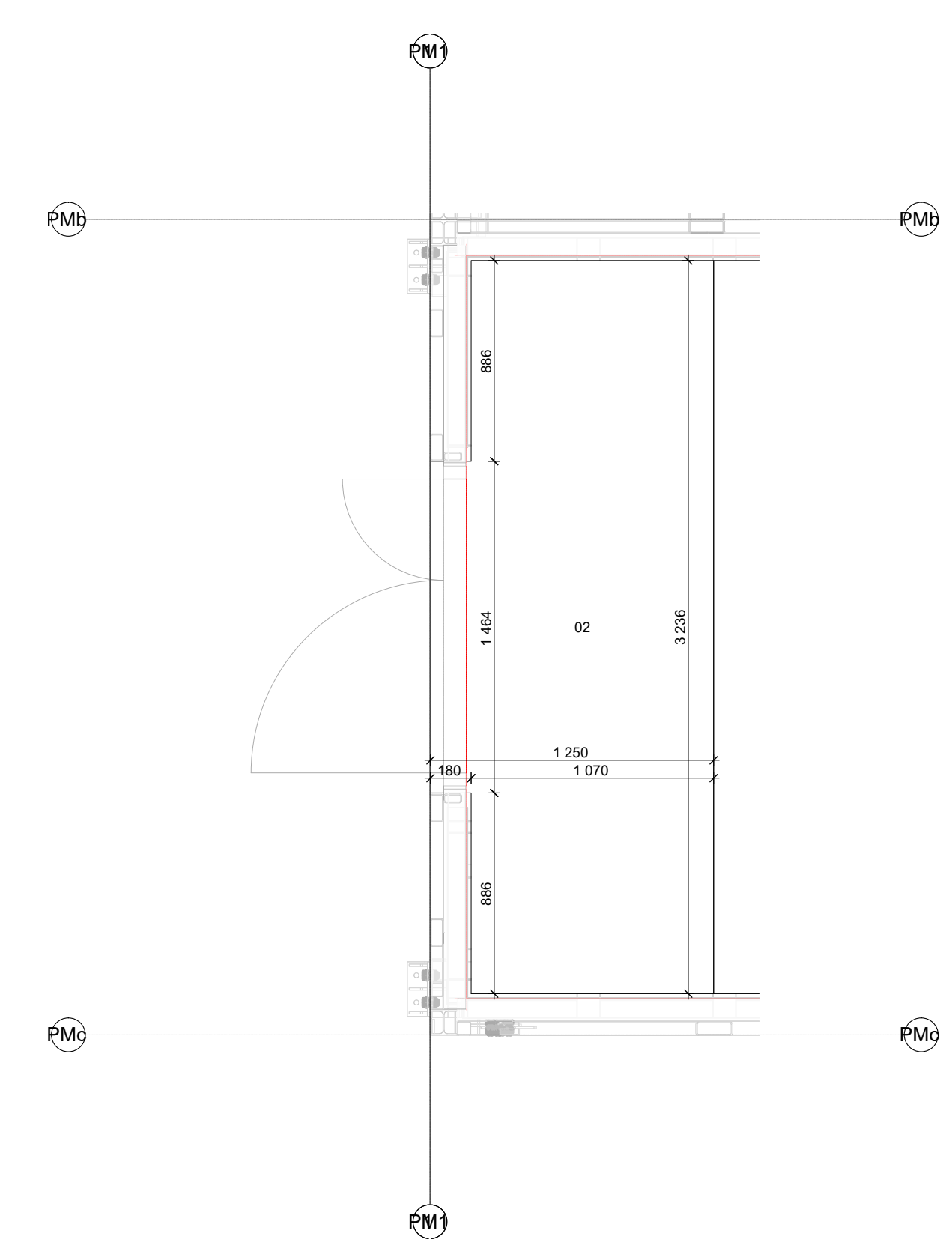
02 PM - Floor Plan - Cement Fibre - Board pos. 02 1 : 25
