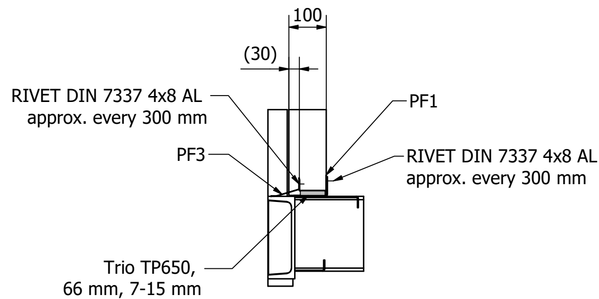
Typical detail B ( 1 : 10 )
