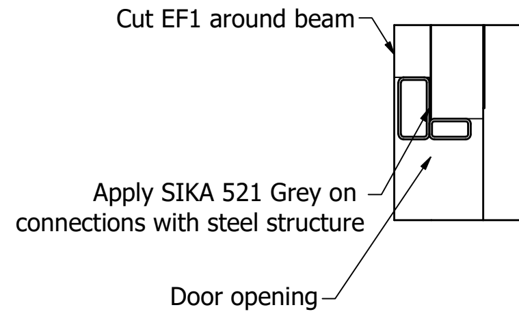
Typical door detail J ( 1 : 10 )
