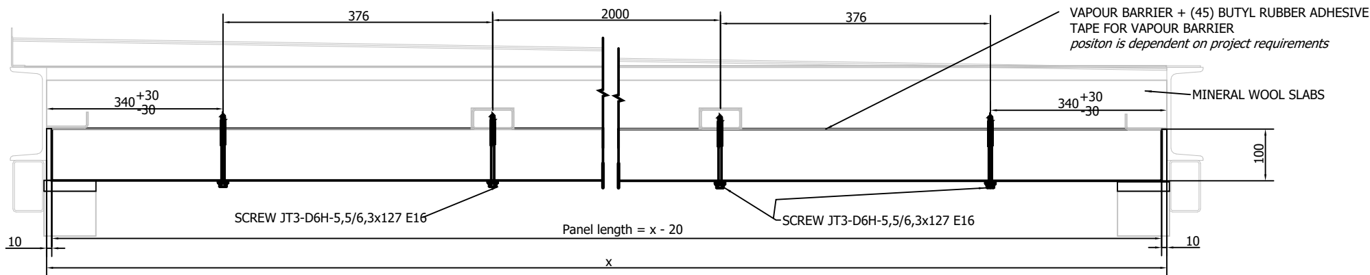
1 PM - Ceiling Layout - Ceiling Panel 100 Copy 2 1 : 50
