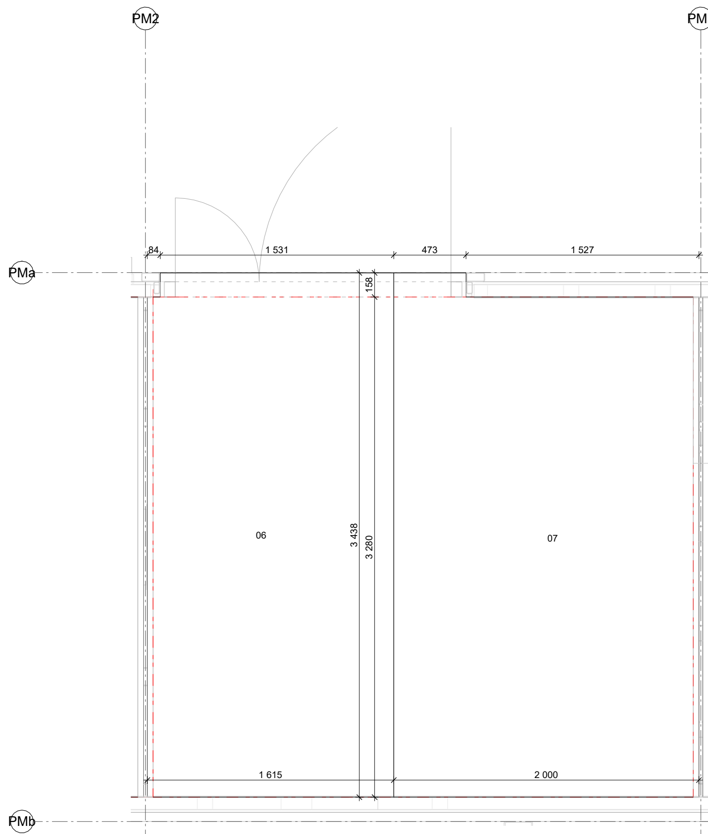
6/7 PM - Floor Plan - Vinyl - Board pos. 06/07 Copy 1 1:25
