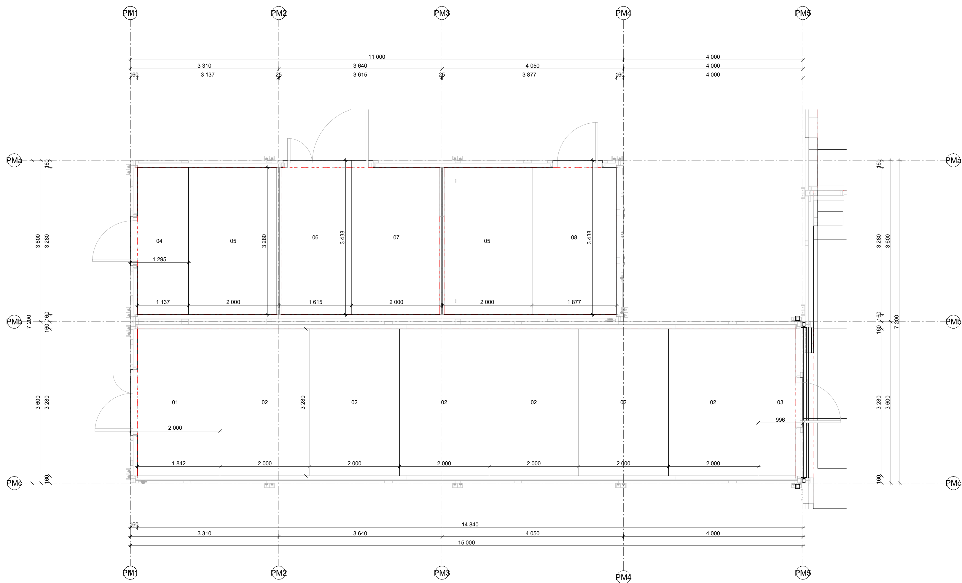
1 PM - FIRST FLOOR LAYER LAYOUT - VINYL 1:50
