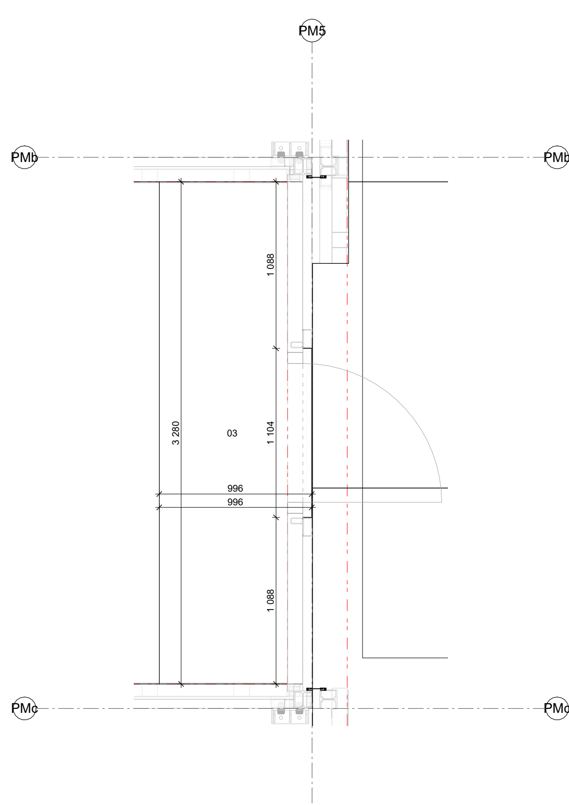
3 PM - Floor Plan - Vinyl - Board pos. 03 Copy 1 1:25
