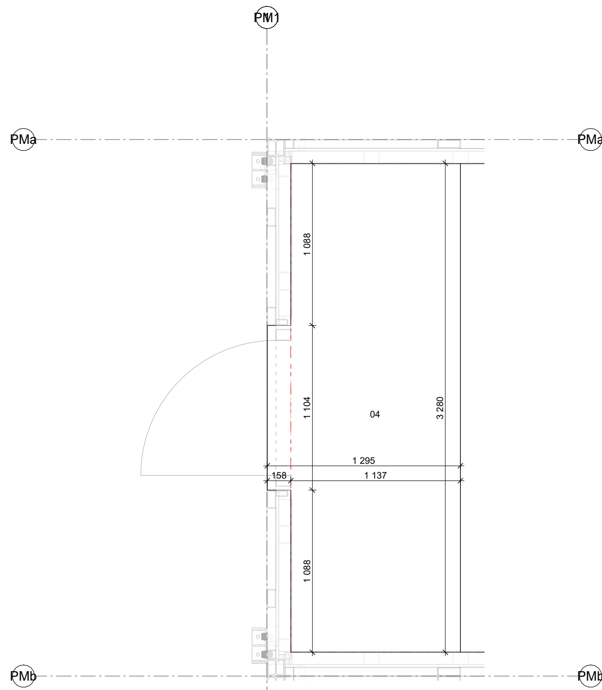
4 PM - Floor Plan - Vinyl - Board pos. 04 Copy 1 1:25
