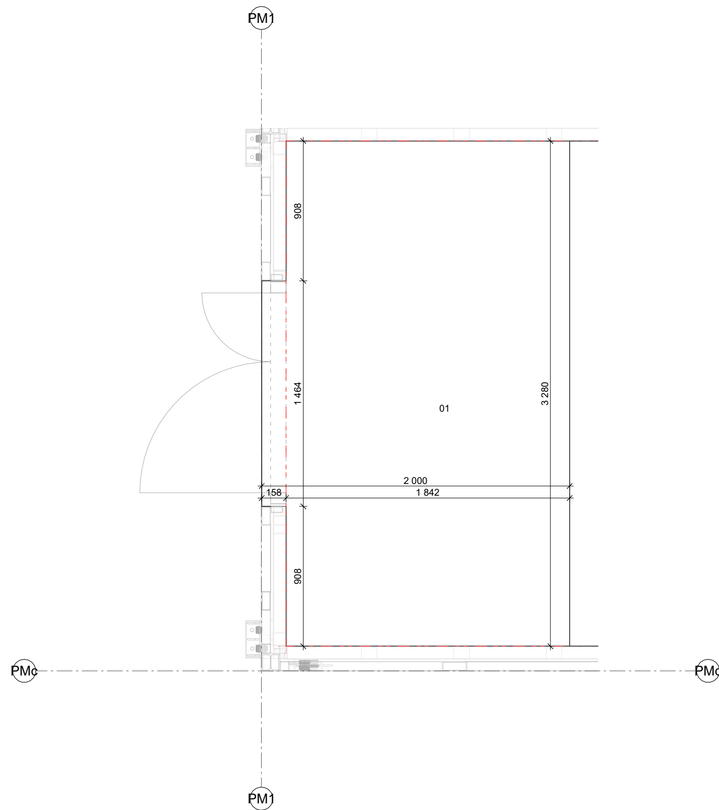
01 PM - Floor Plan - Vinyl - Board pos. 01 Copy 1 1:25
