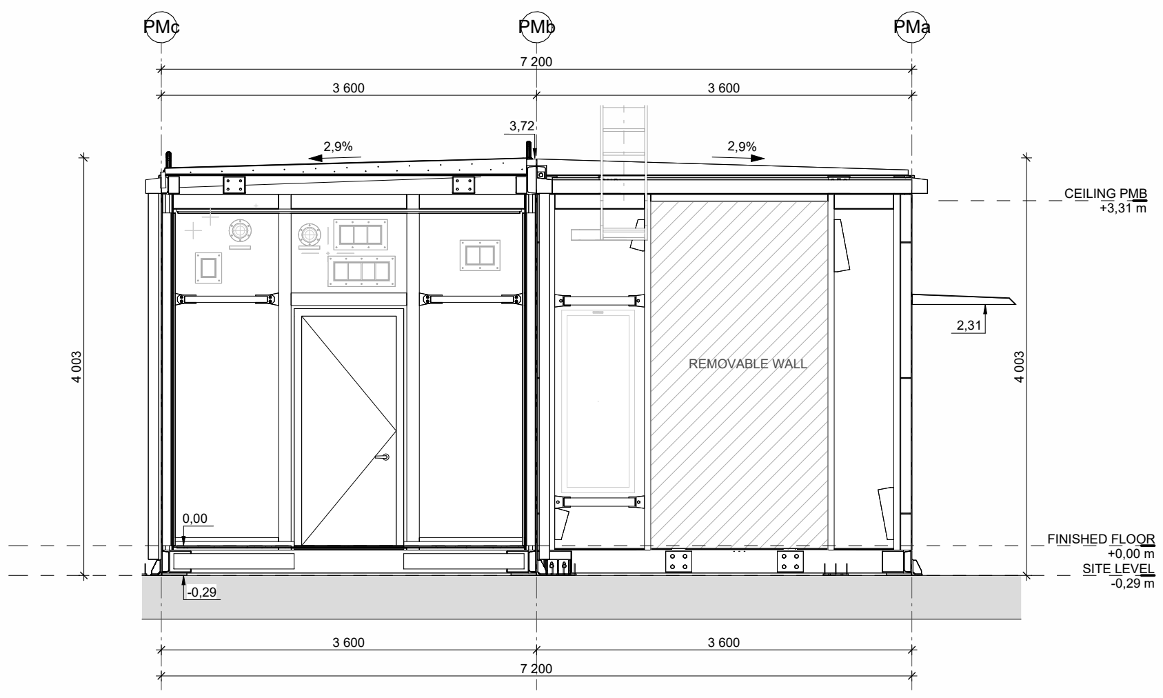
5 PM+MV - ELEVATION EAST 1 : 50
