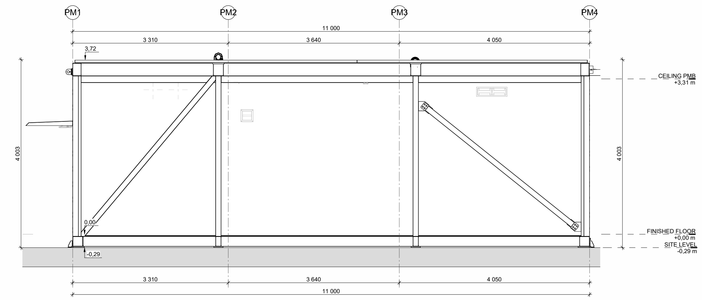
3 MV - ELEVATION SOUTH 1 : 50
