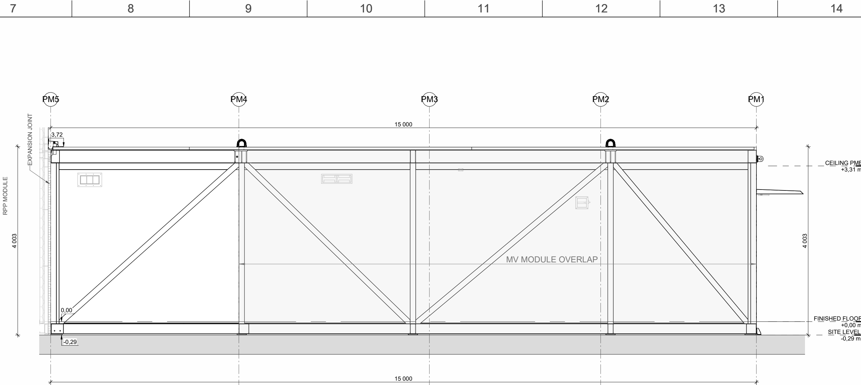
2 PM - ELEVATION NORTH 1 : 50
