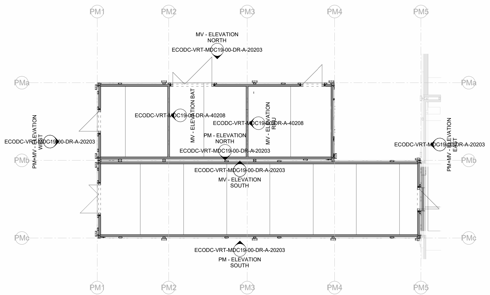
KEY PLAN - POWER MODULE ELEVATION POSITIONS 1 : 100
