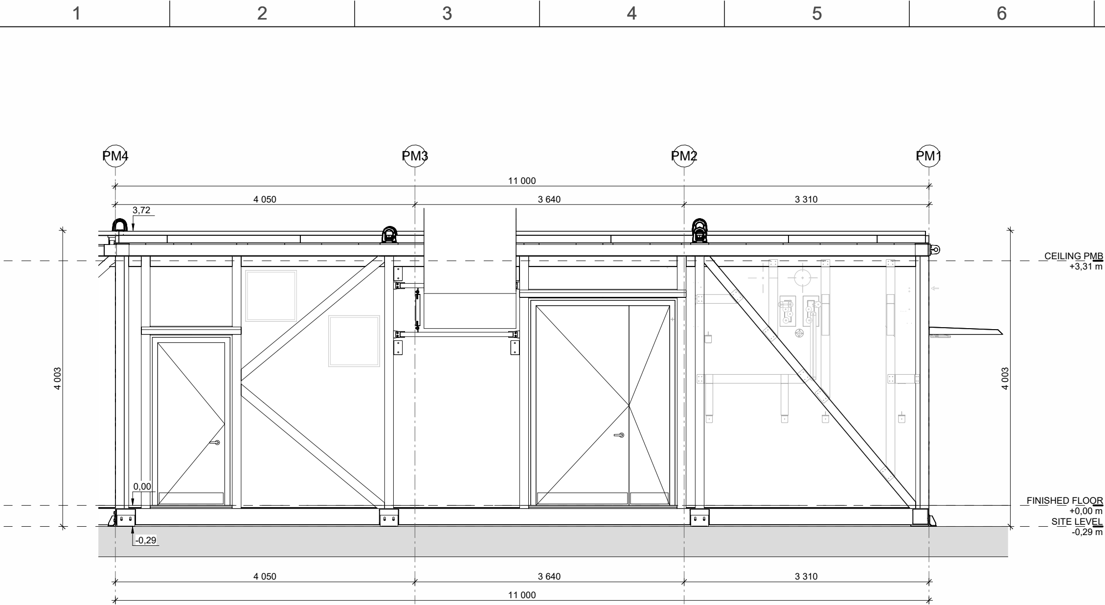
1 MV - ELEVATION NORTH 1 : 50
