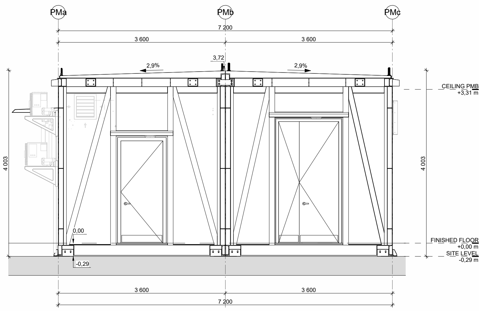
6 PM+MV - ELEVATION WEST 1 : 50
