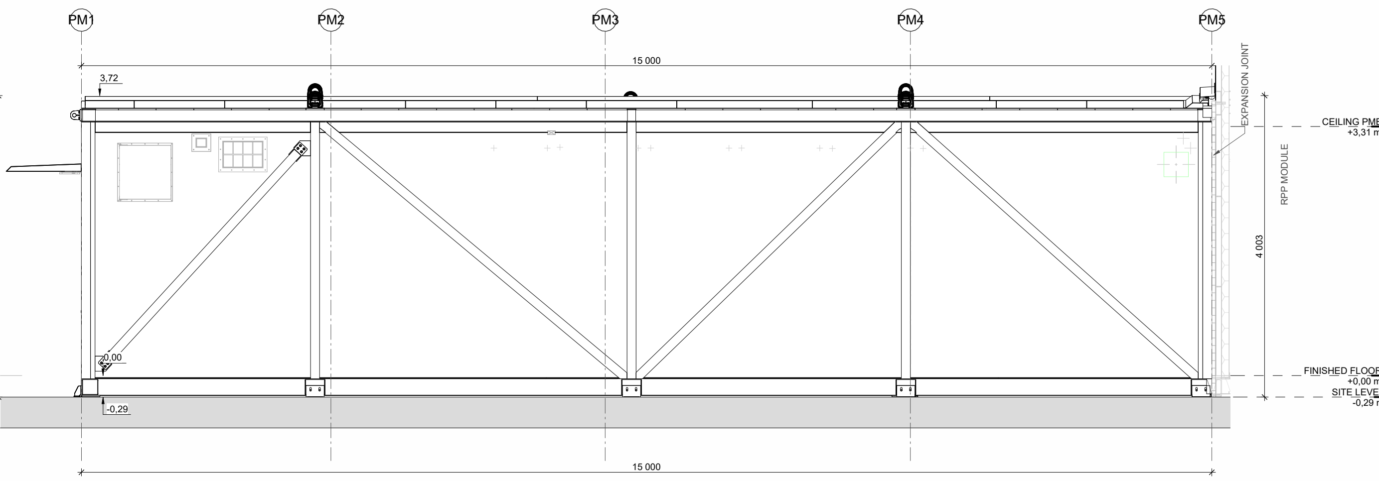
4 PM - ELEVATION SOUTH 1 : 50
