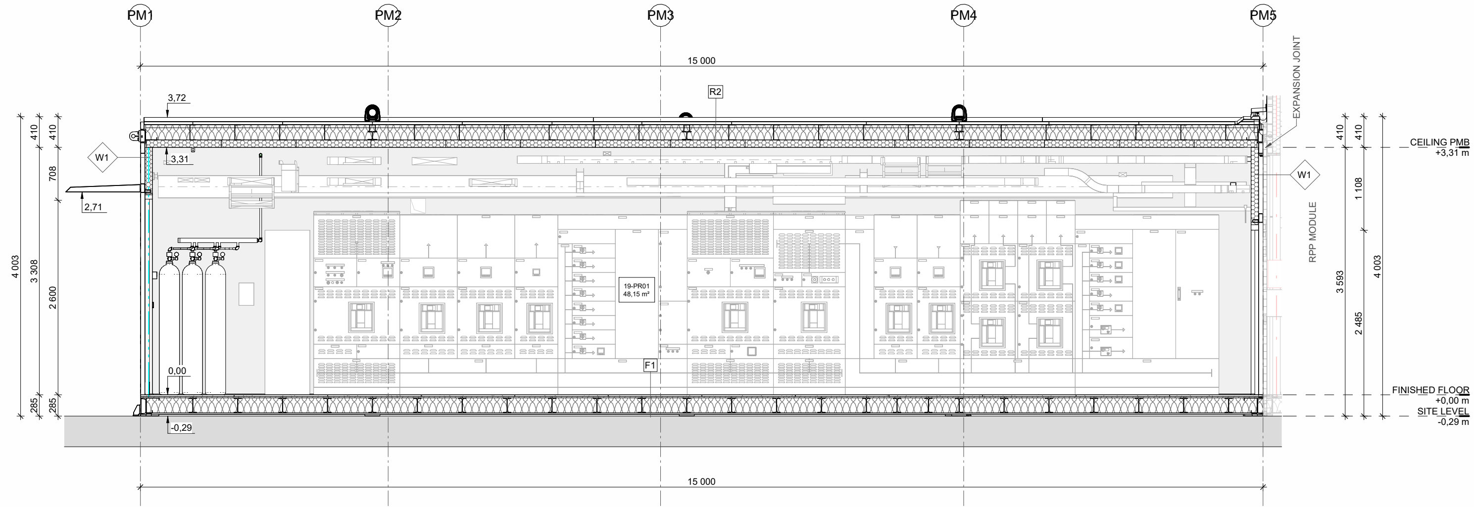
3 POWER MODULE - SECTION C-C 1:50
