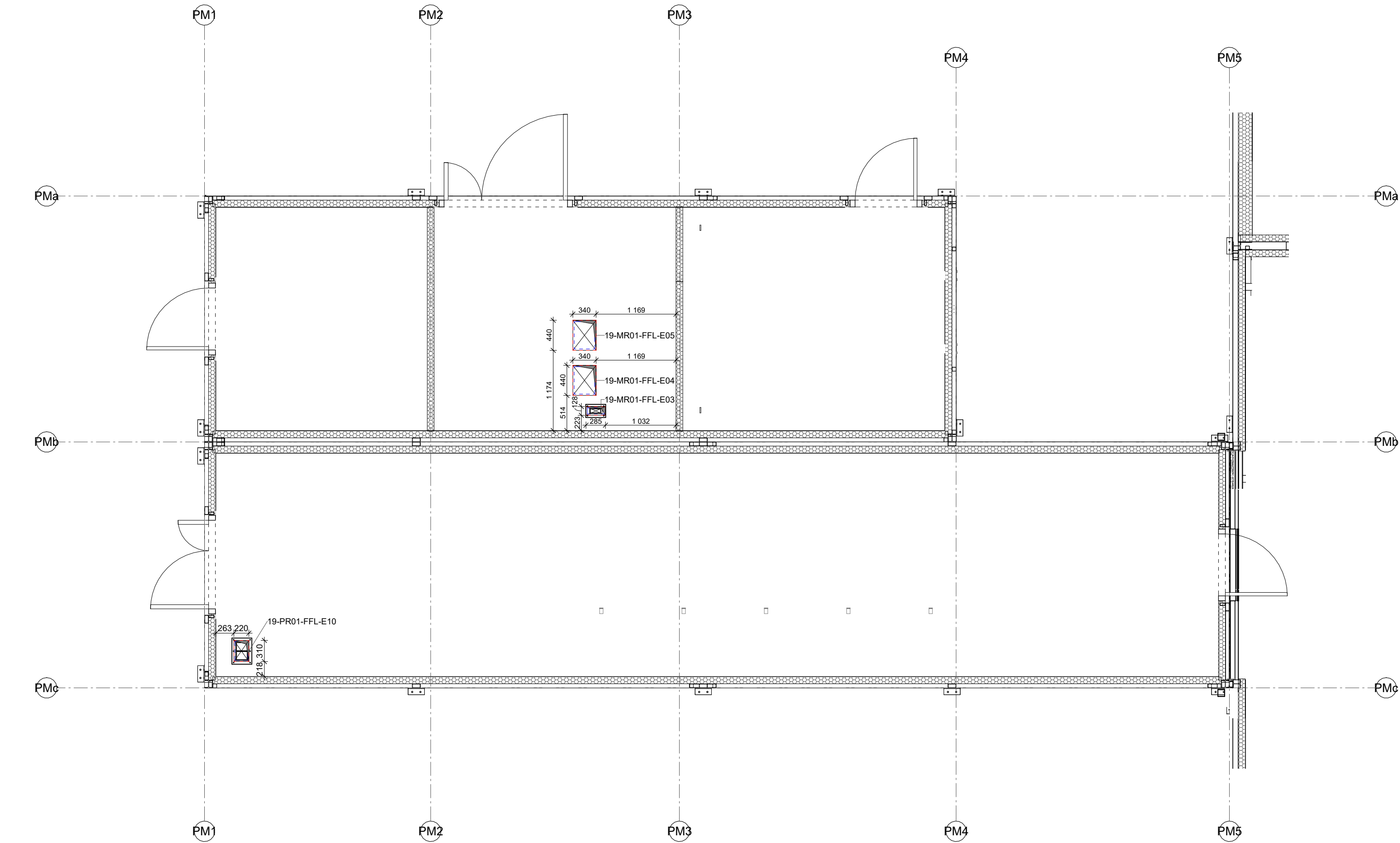
1 ARCHITECTURAL BUILDING PENETRATIONS – POWER MODULE – FLOOR PLAN 1 : 50
