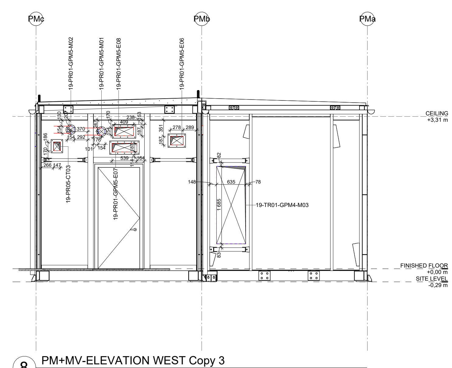
8 PM+MV-ELEVATION WEST Copy 3 1 : 50
