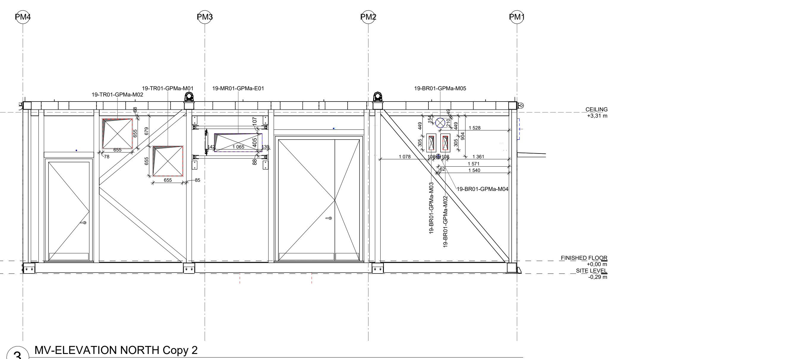
3 MV-ELEVATION NORTH Copy 2 1 : 50
