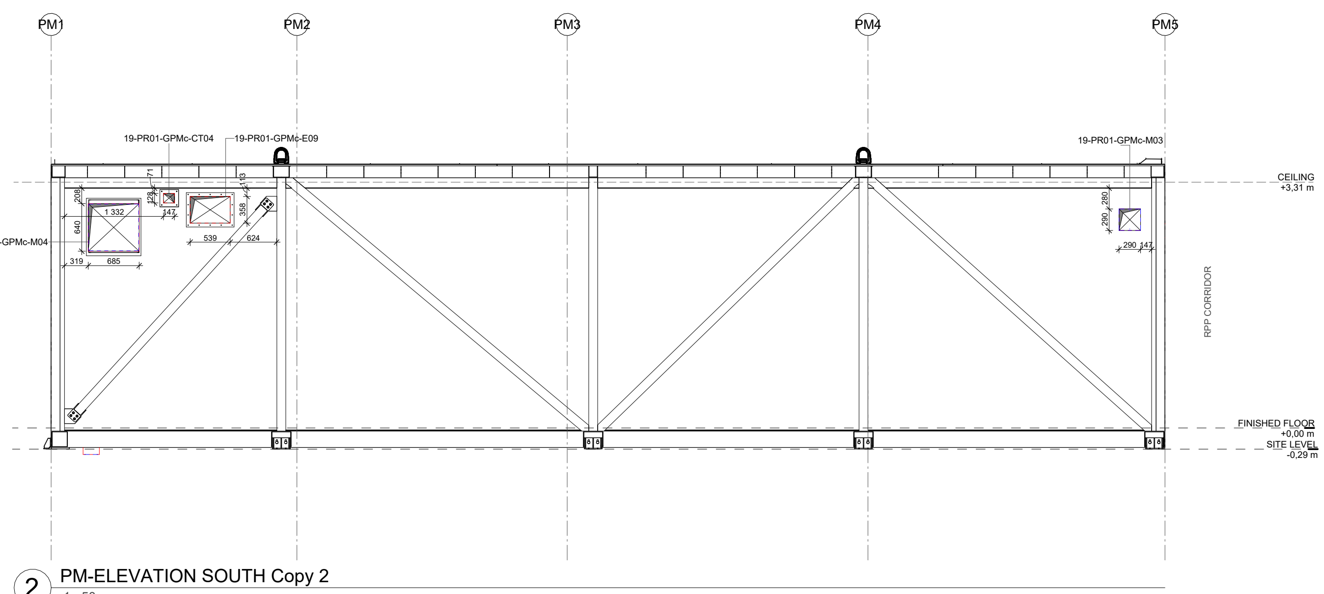
2 PM-ELEVATION SOUTH Copy 2 1 : 50
