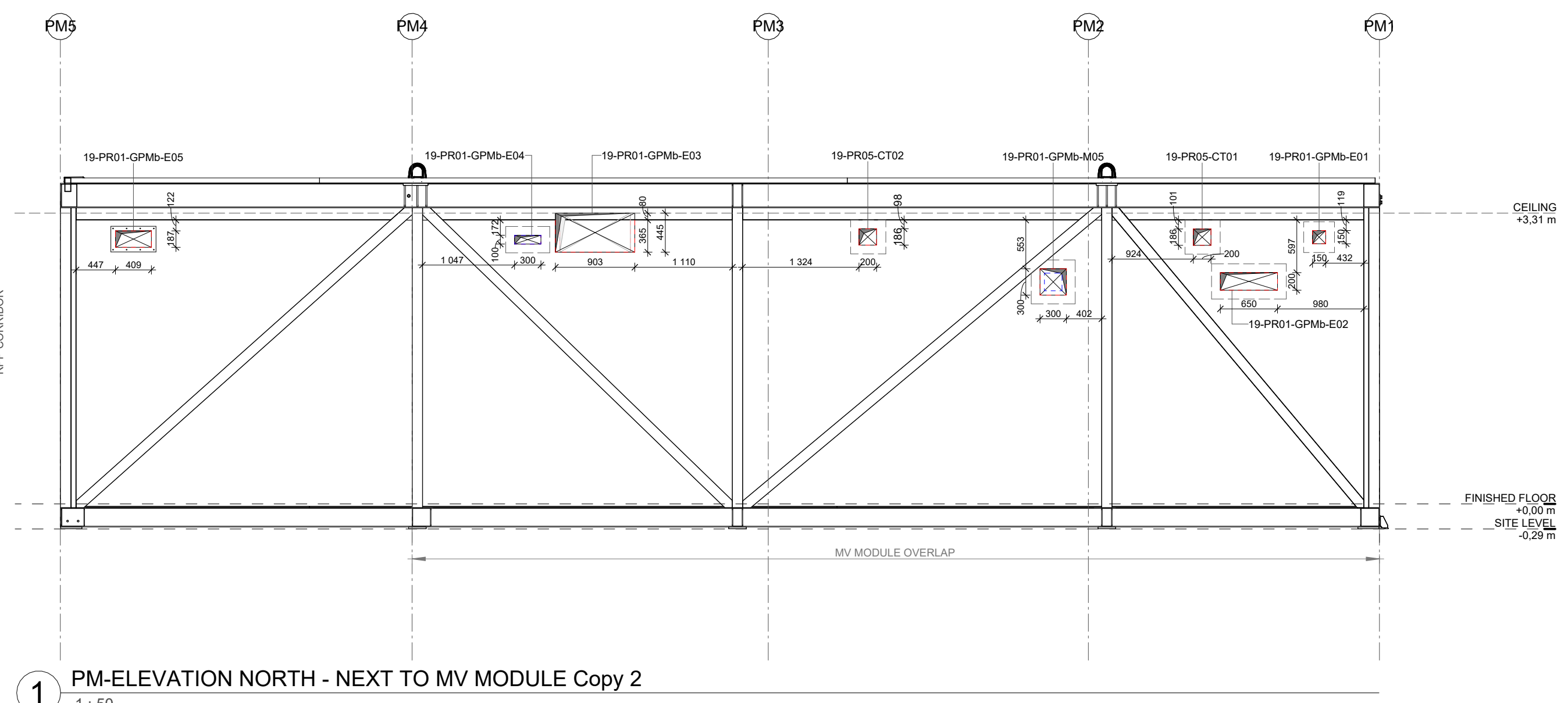
1 PM-ELEVATION NORTH - NEXT TO MV MODULE Copy 2 1 : 50
