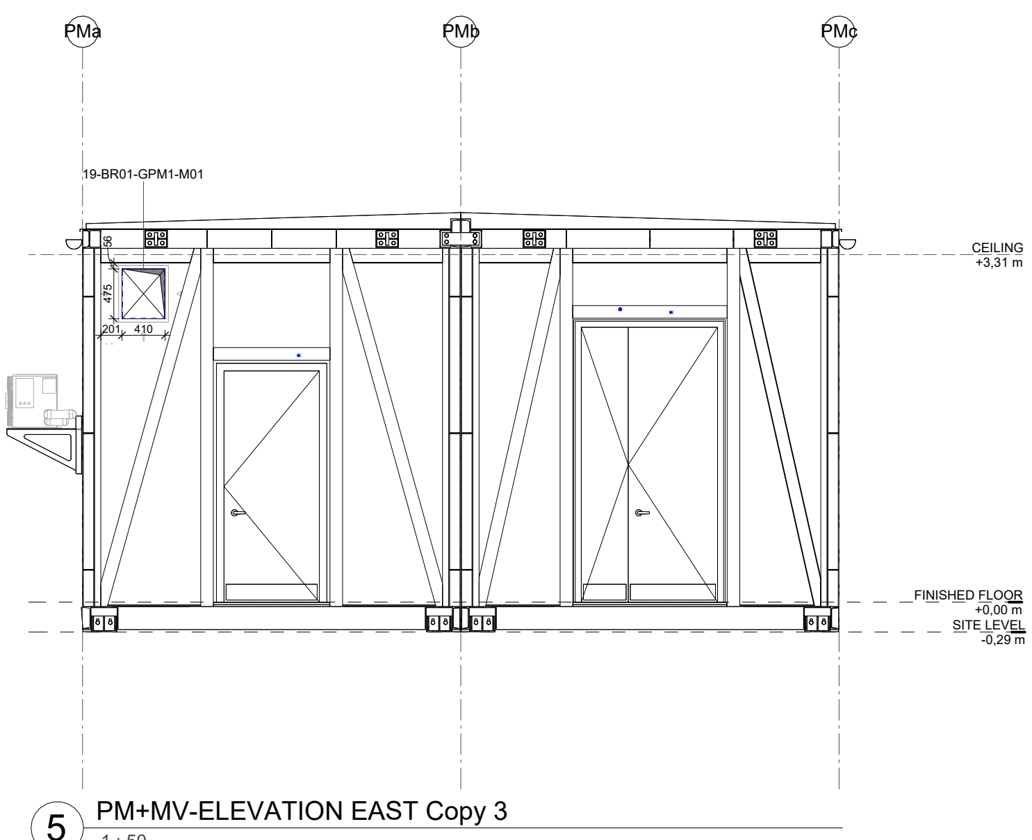
5 PM+MV-ELEVATION EAST Copy 3 1 : 50
