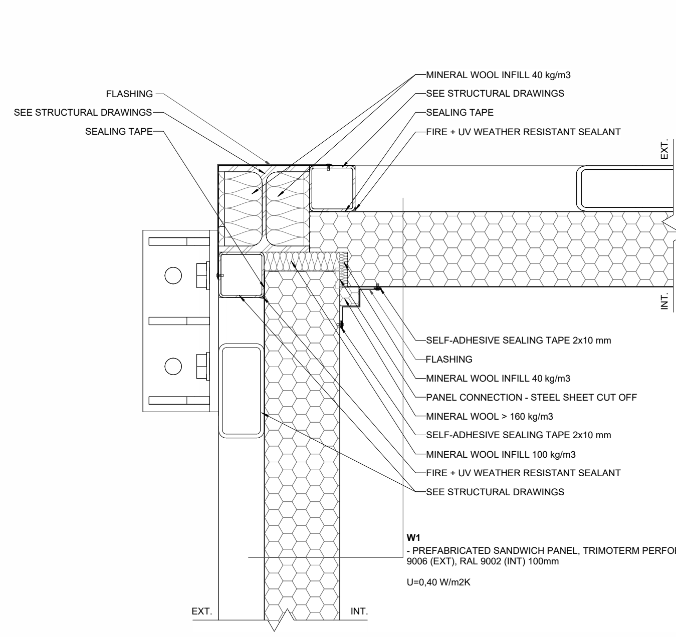
H01 MV/MS - MODULE CORNER 1:5
