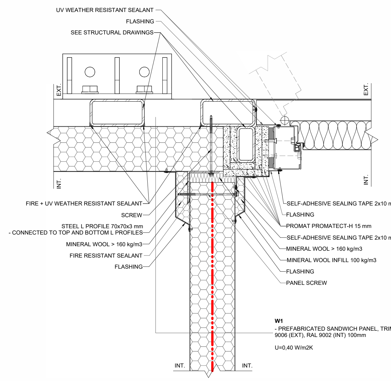
H02 MV - INT./EXT. WALL CONNECTION 1:5
