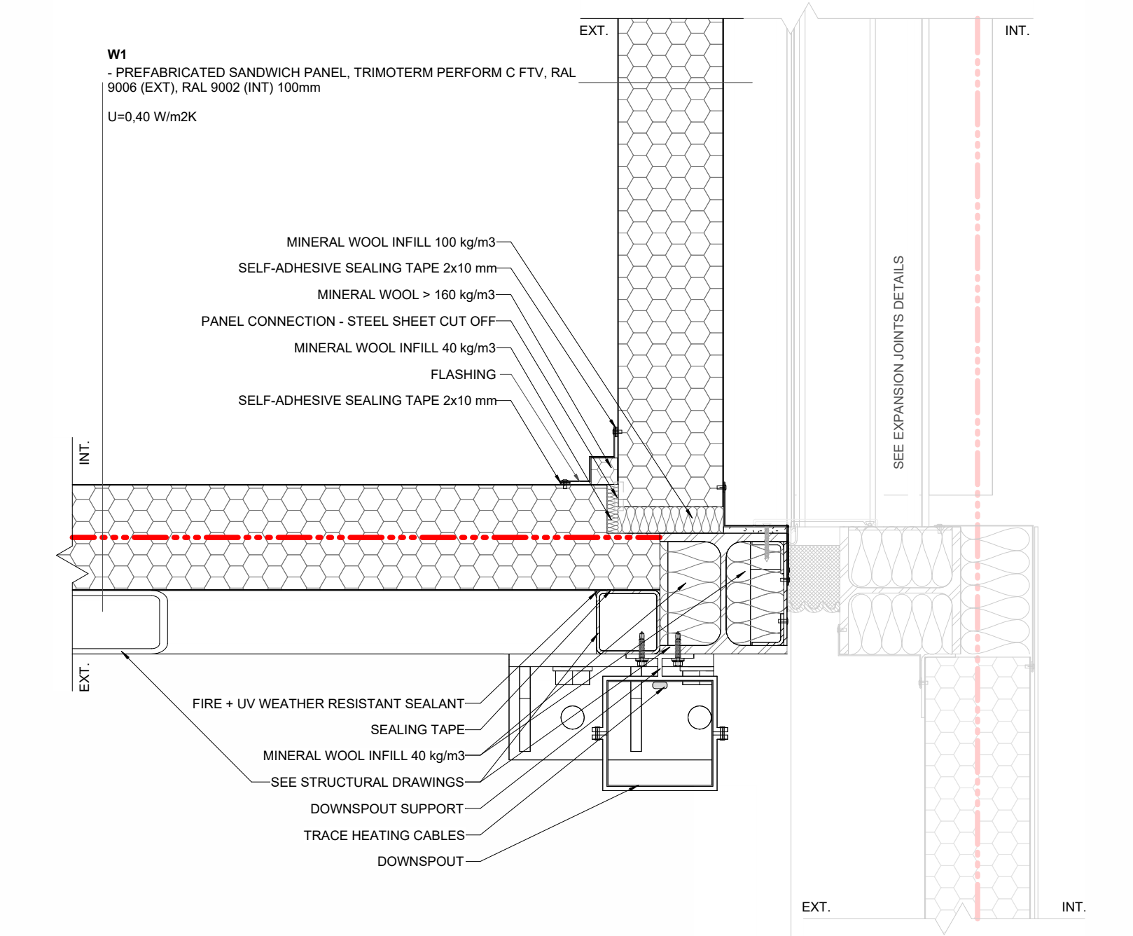
H10 PM - MODULE CORNER, RPP MODULE CONNECTION 1:5
