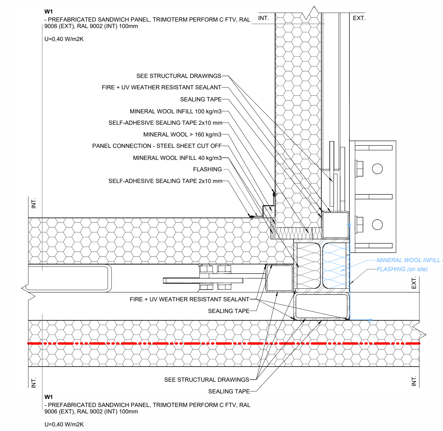
H07 MV - MODULE CORNER, PM MODULE CONNECTION 1:5
