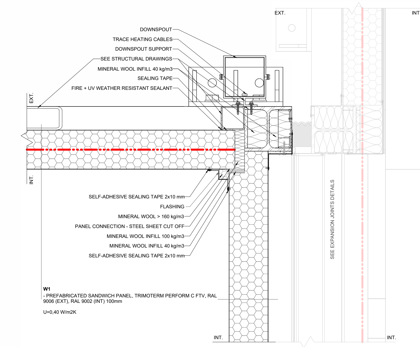
H08 PM - MODULE CORNER, RPP MODULE CONNECTION 1:5
