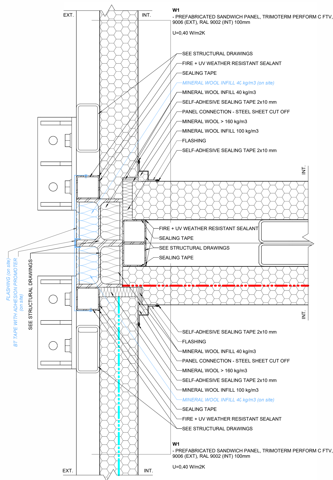
H05 PM/MV - MODULE CONNECTION 1:5
