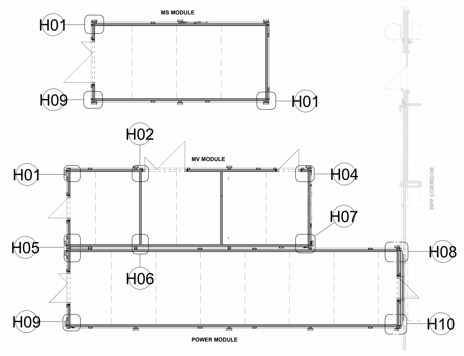
KEY PLAN - PM/MV/MS MODULE DETAIL POSITIONS - HORIZONTAL VIEWS
