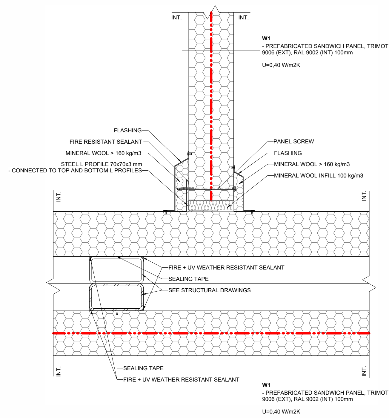
H06 MV - INT./EXT. WALL CONNECTION 1:5
