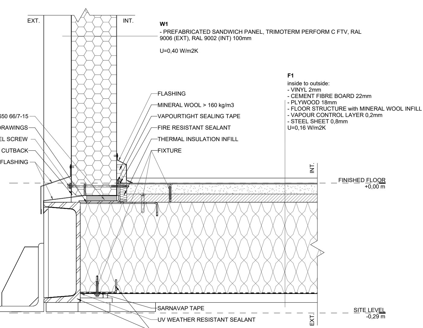
V02 PM/MV/MS - EXT. WALL/FLOOR CONNECTION 1:5
