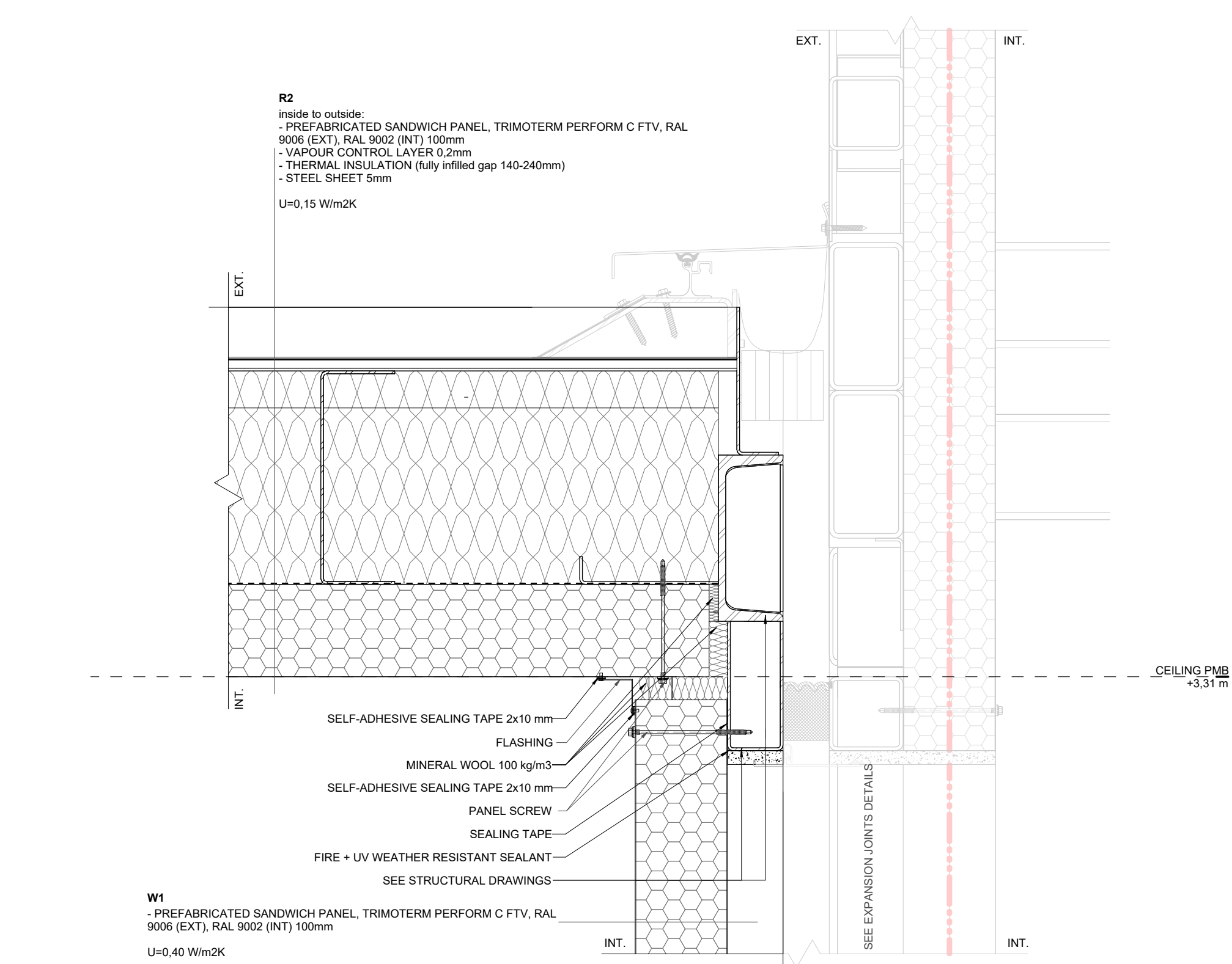
V11 PM - RPP MODULE CONNECTION-ROOF 1:5
