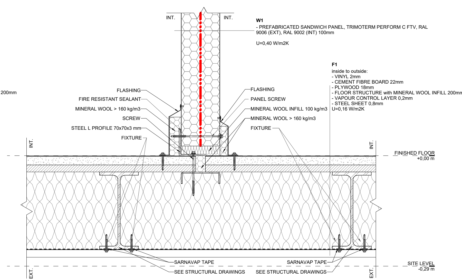
V04 MV - INT. WALL/FLOOR CONNECTION 1:5
