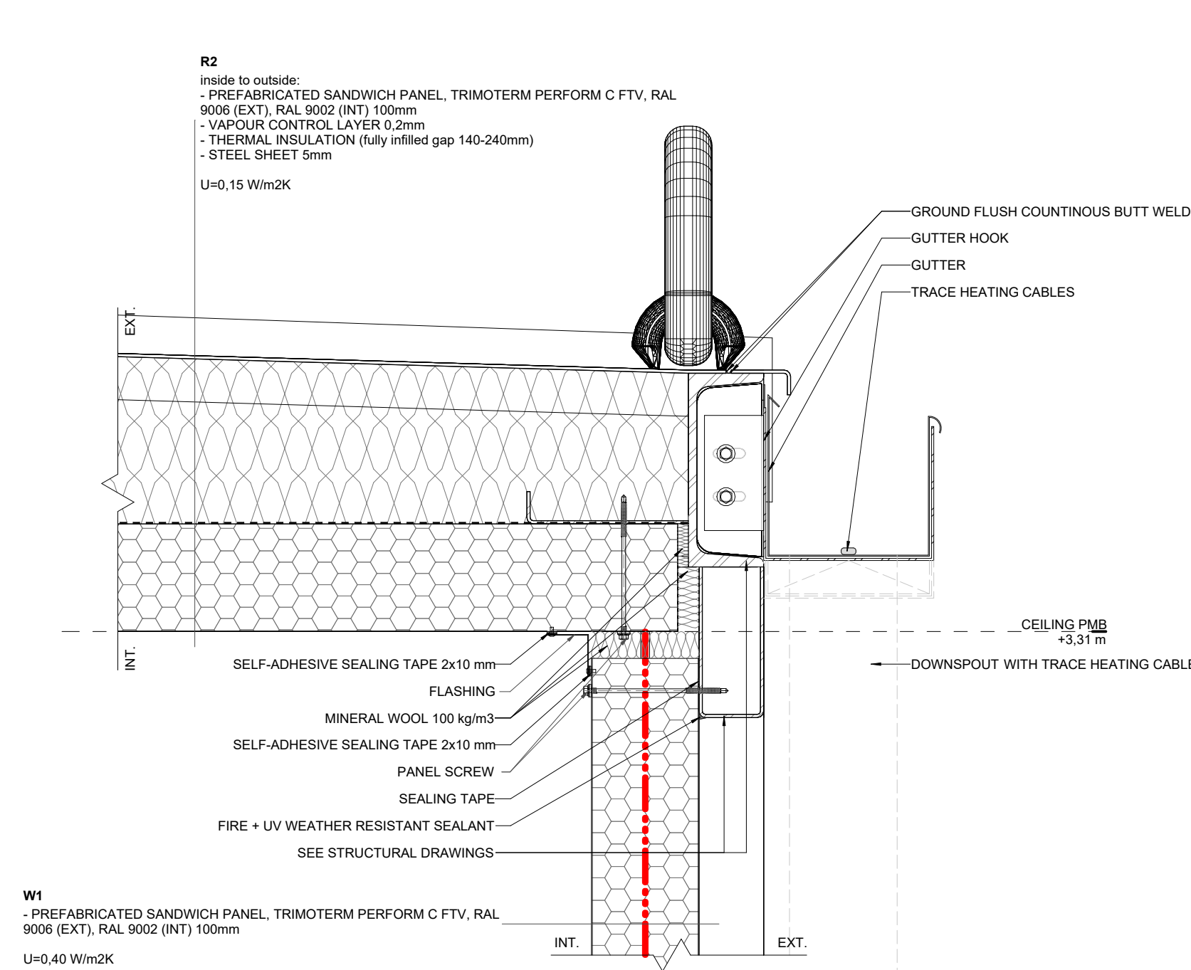
V09 PM/MV/MS - EXT. WALL/ROOF CONNECTION 1:5
