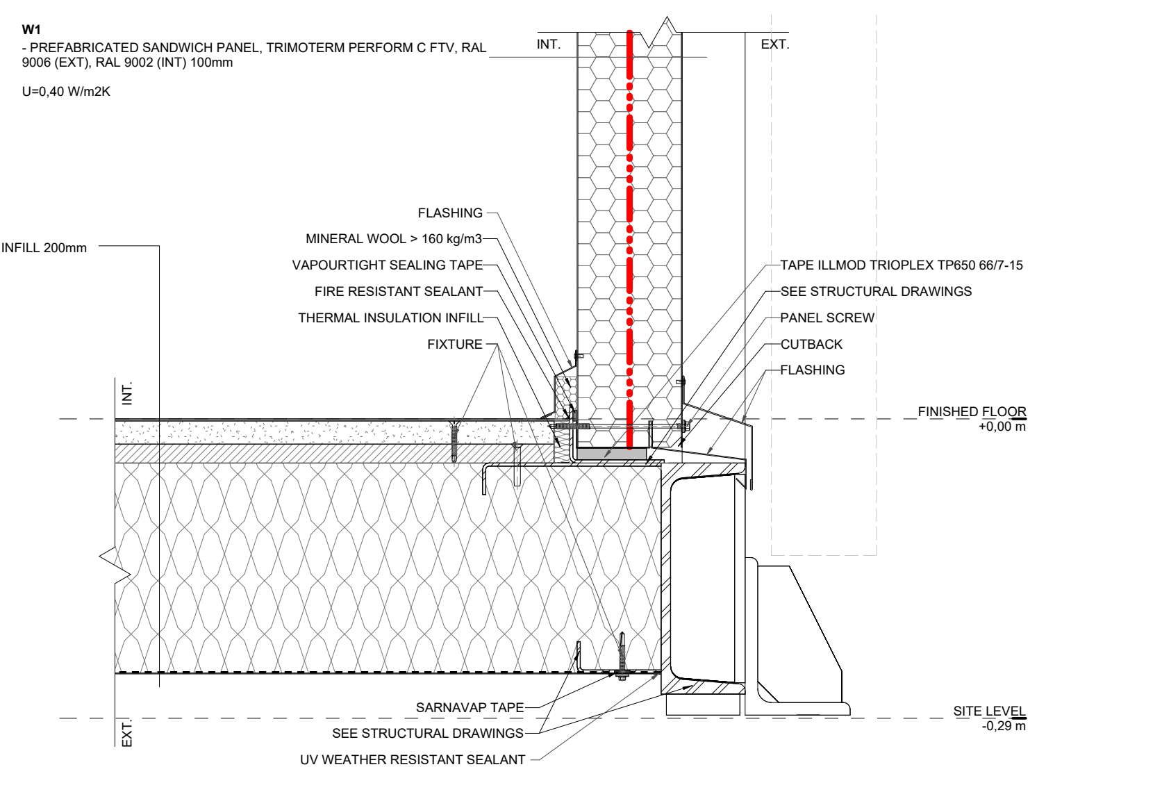
V10 PM/MV/MS - EXT. WALL/FLOOR CONNECTION 1:5
