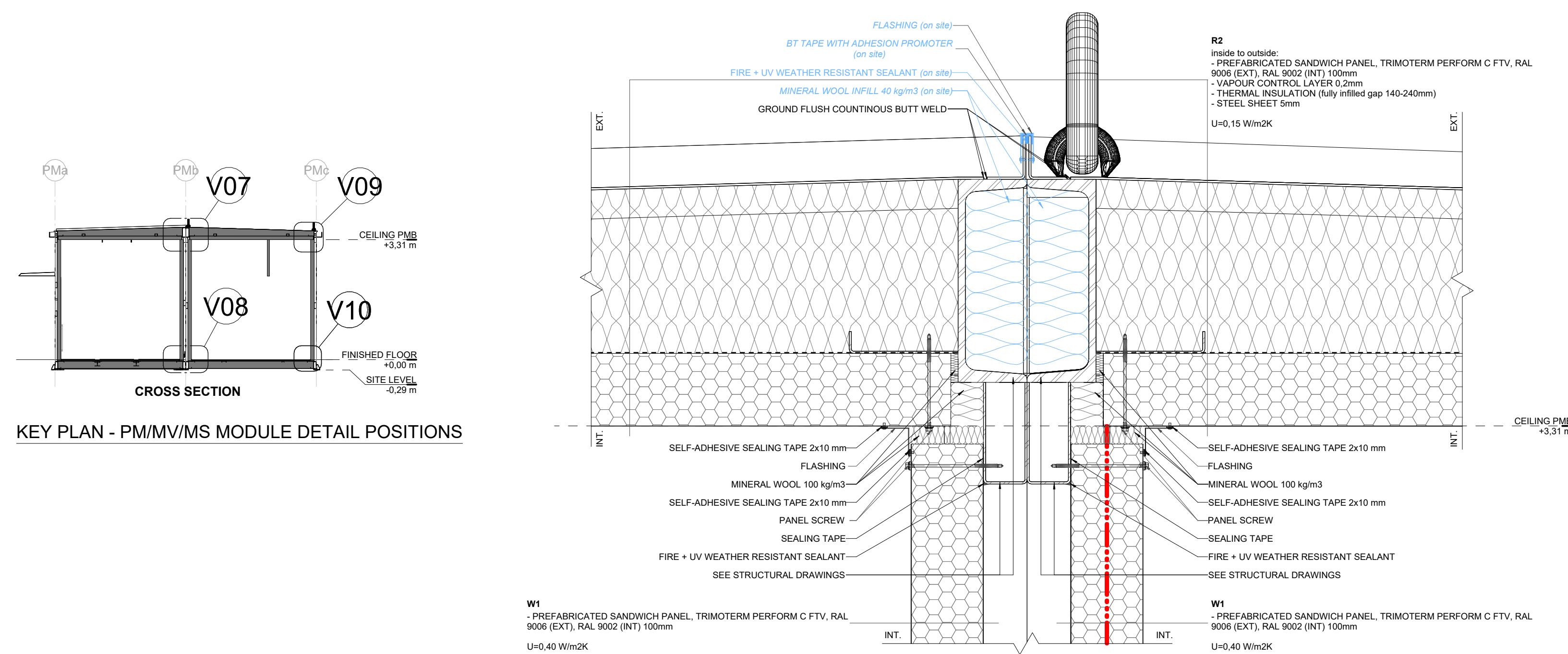
V07 PM/MV - MODULE CONNECTION-ROOF 1:5
