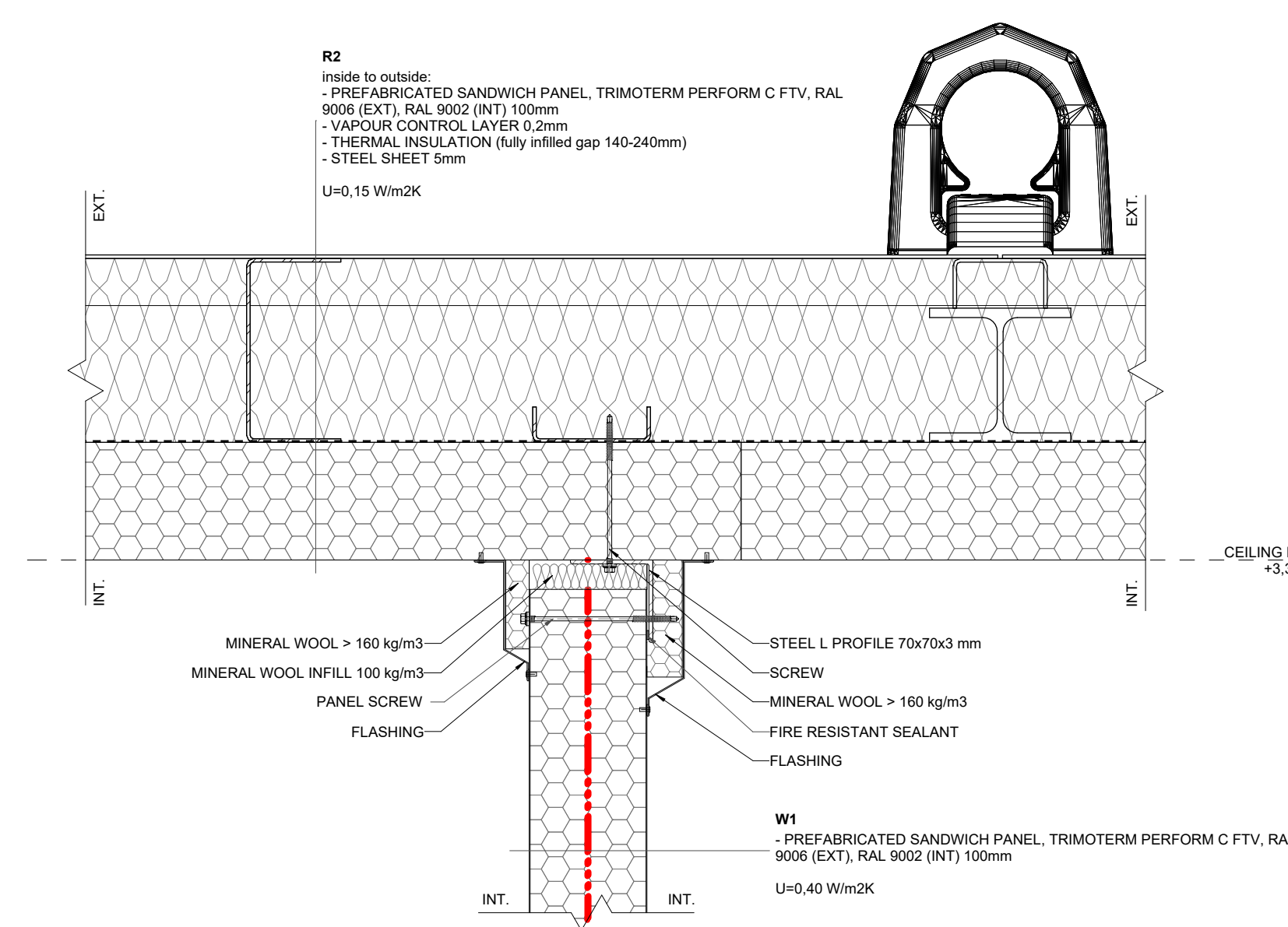
V05 MV - INT. WALL/ROOF CONNECTION 1:5
