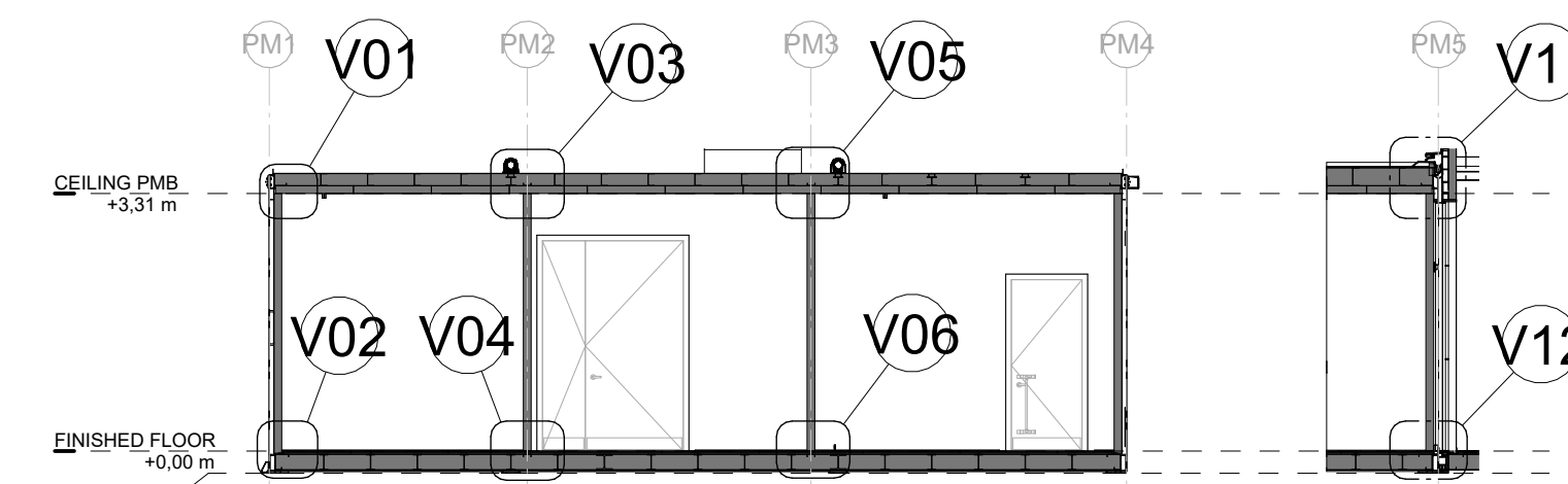
LONGITUDINAL SECTION KEY PLAN - PM/MV/MS MODULE DETAIL POSITIONS - VERTICAL VIEWS
