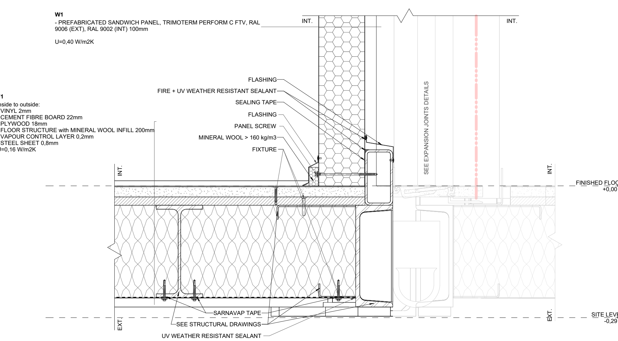
V12 PM - RPP MODULE CONNECTION-FLOOR 1:5
