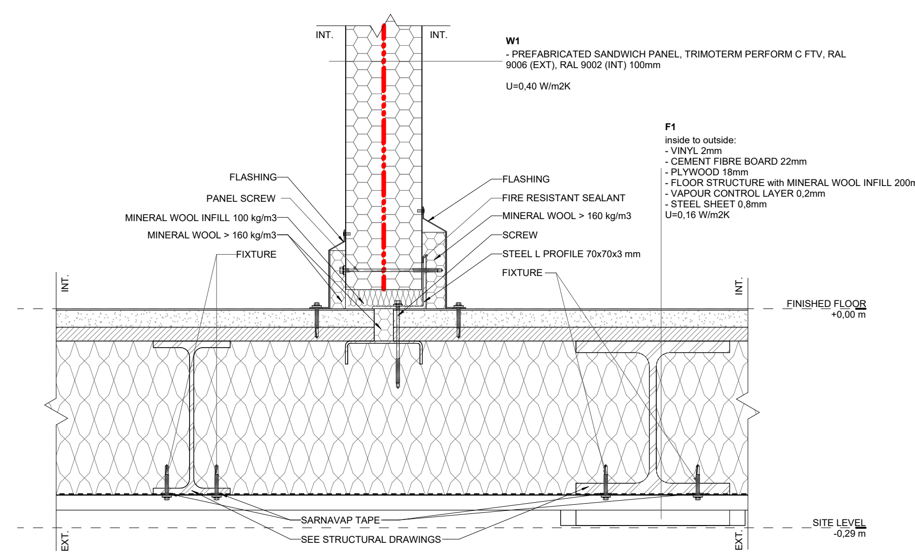
V06 MV - INT. WALL/FLOOR CONNECTION 1:5
