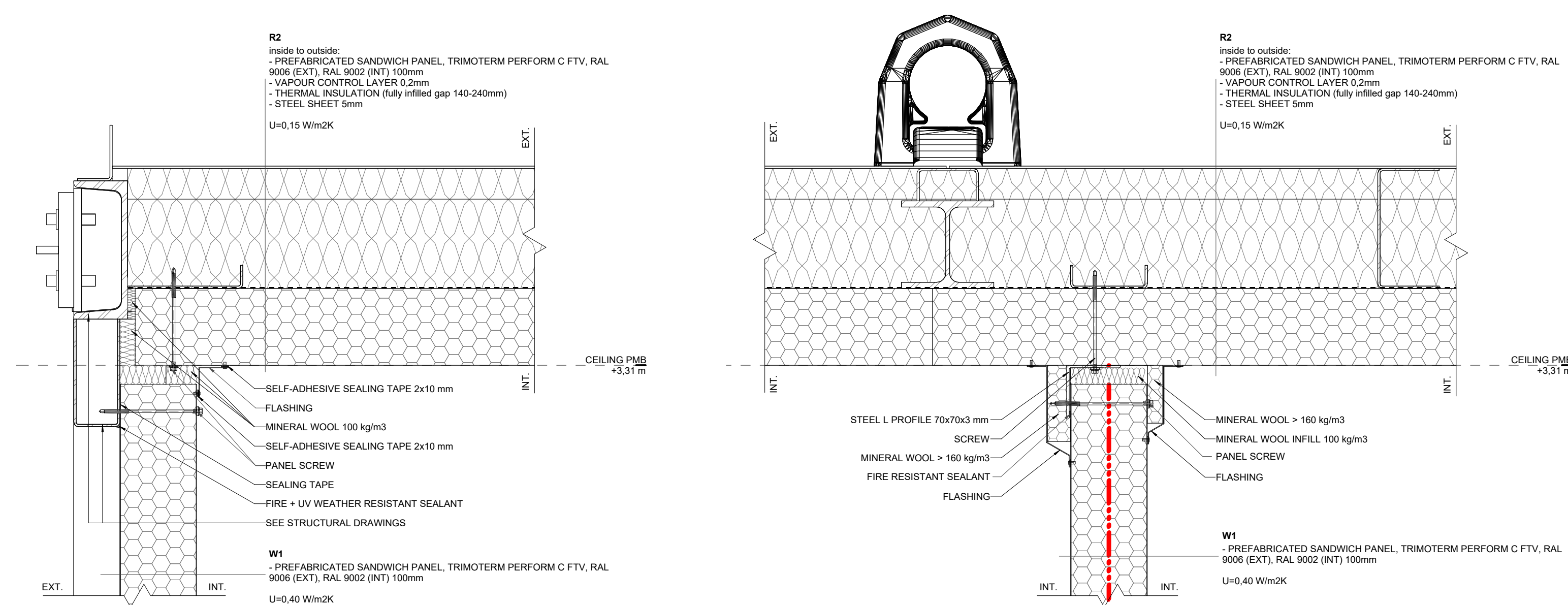
V01 PM/MV/MS - EXT. WALL/ROOF CONNECTION 1:5
