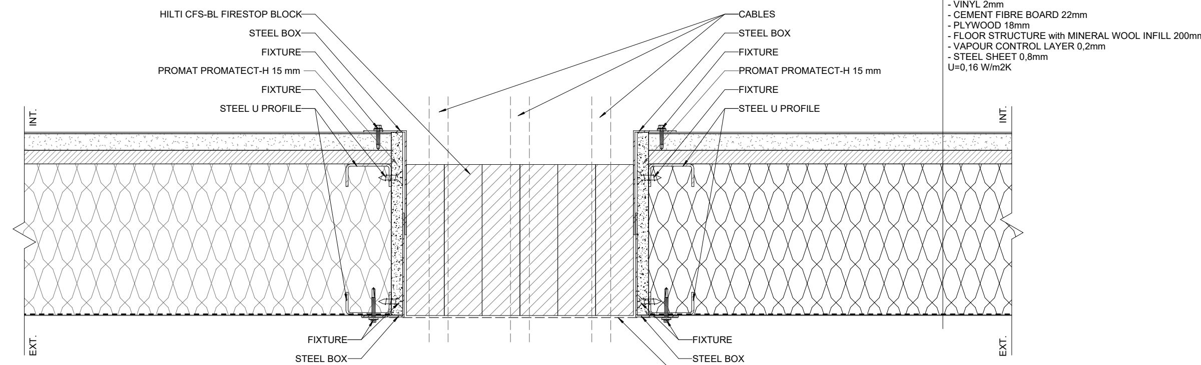
P15 HILTI CFS-BL FIRESTOP BLOCKS - FLOOR 1:5
