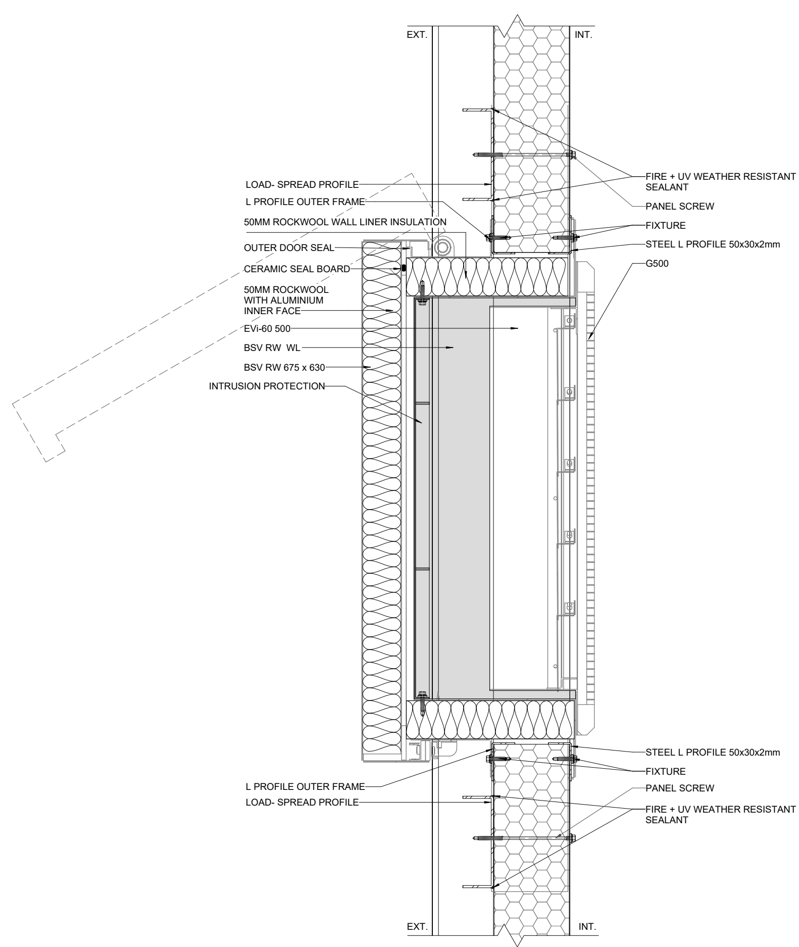
VERTICAL VIEW
