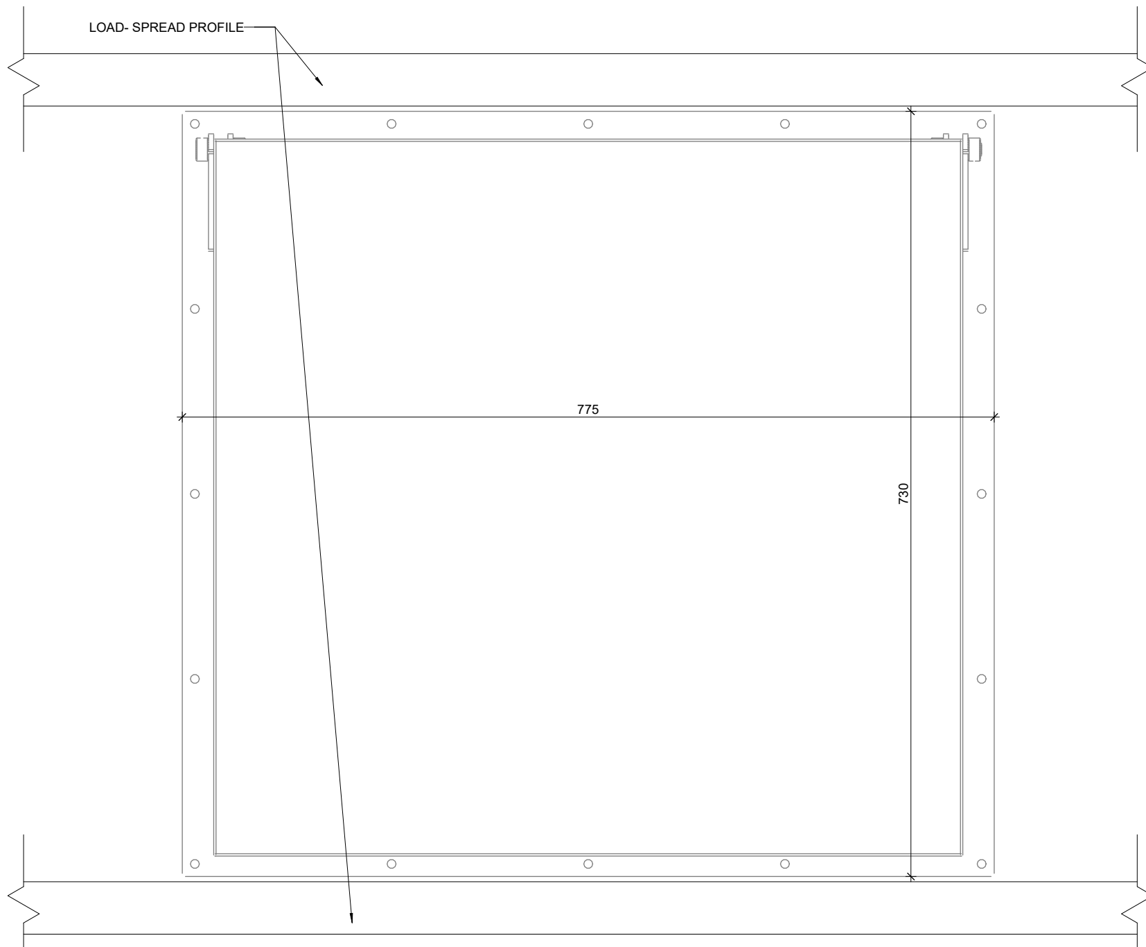
EXTERIOR ELEVATION
