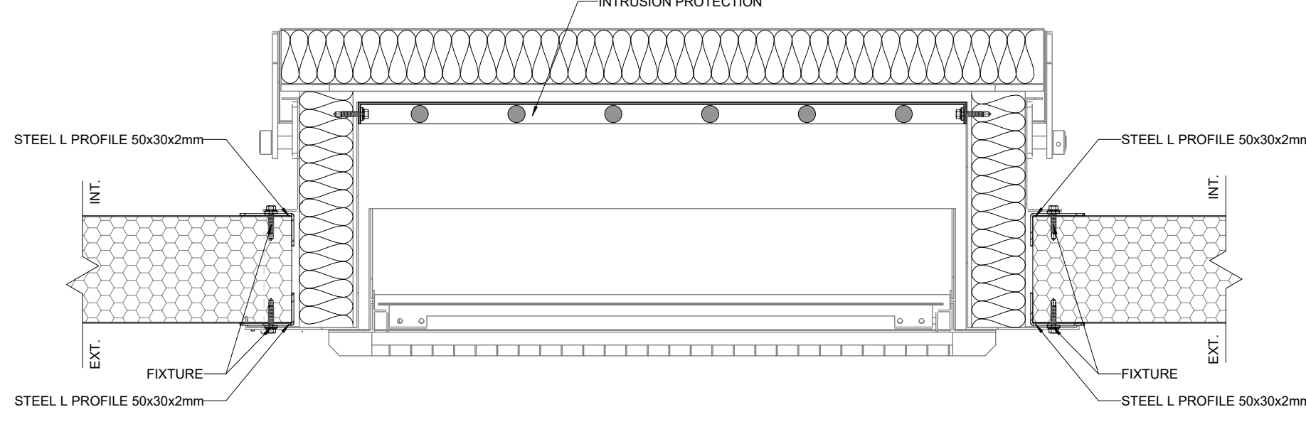
HORIZONTAL VIEW
