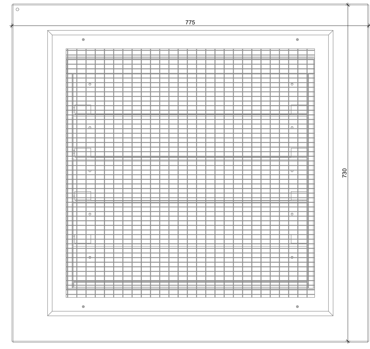
INTERIOR ELEVATION
