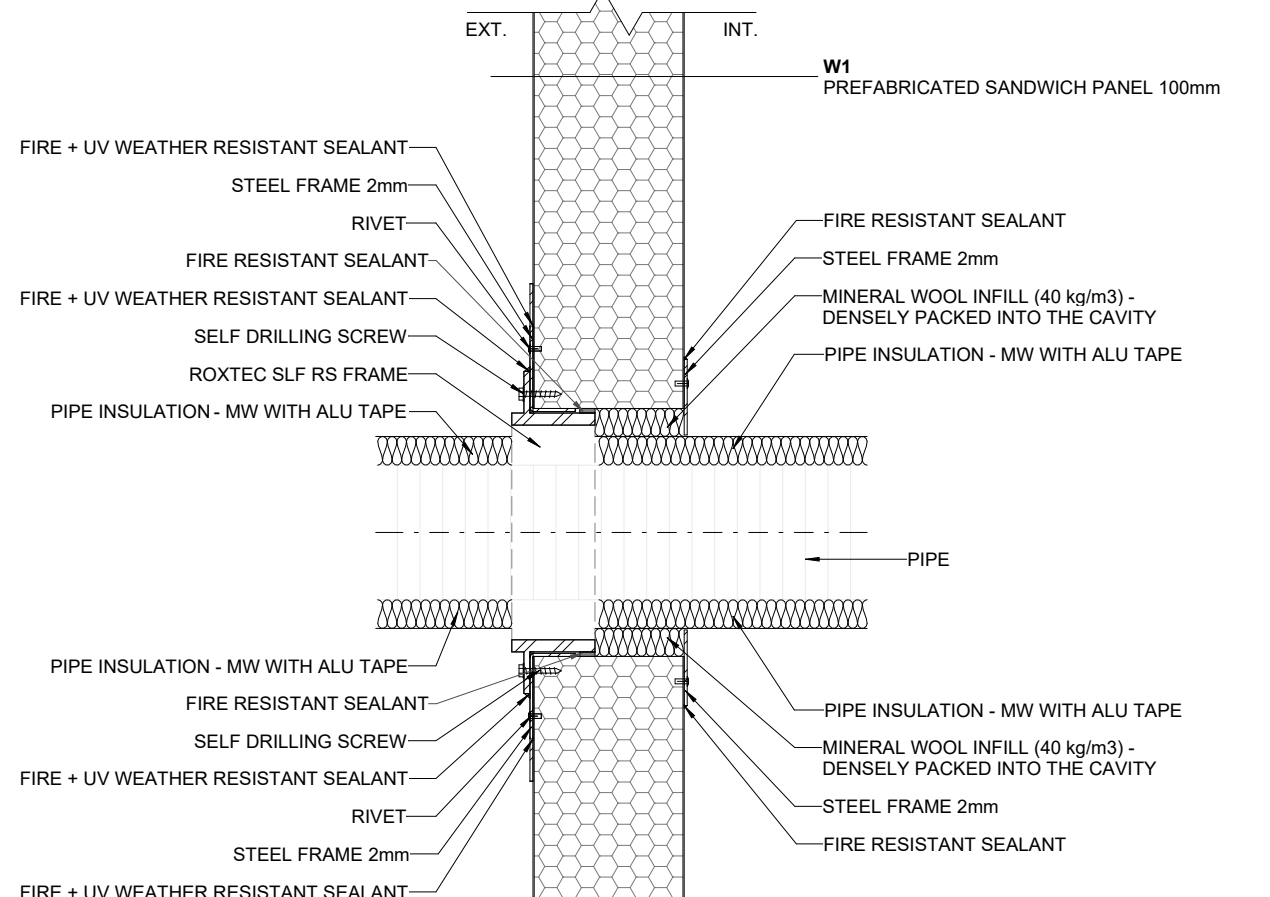
VERTICAL VIEW
