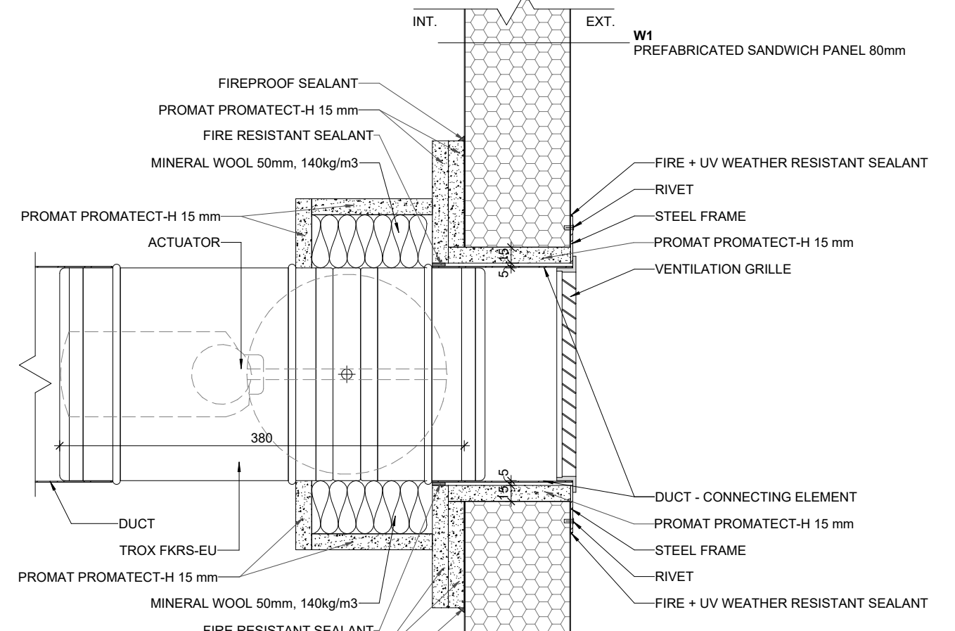
VERTICAL VIEW
