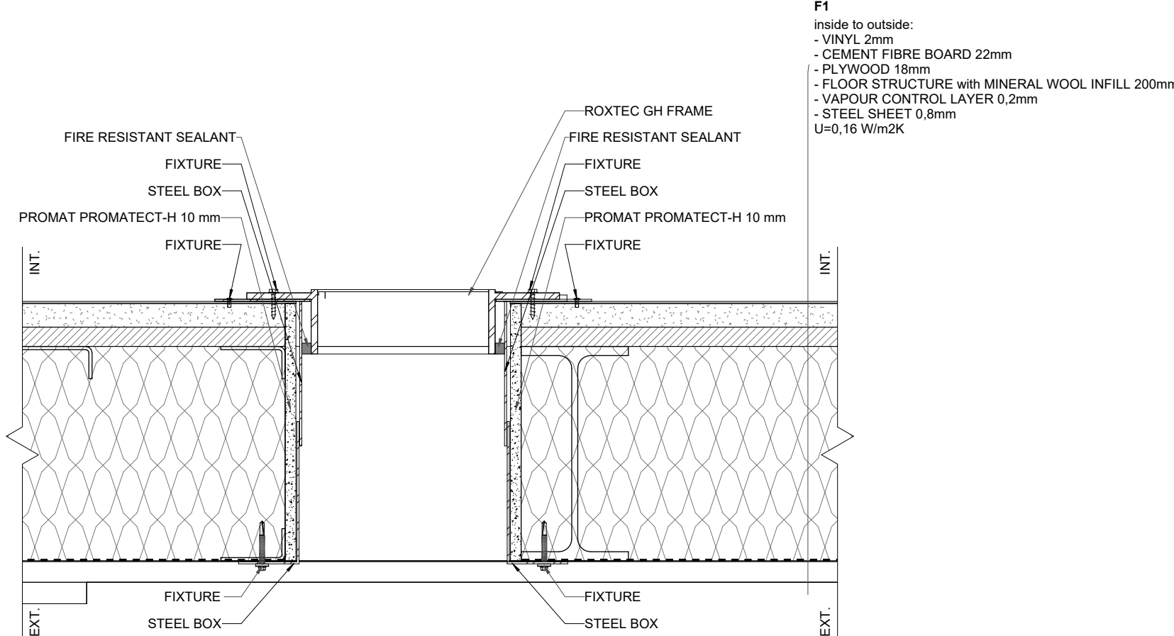
P03 ROXTEC GH - FLOOR 1:5
