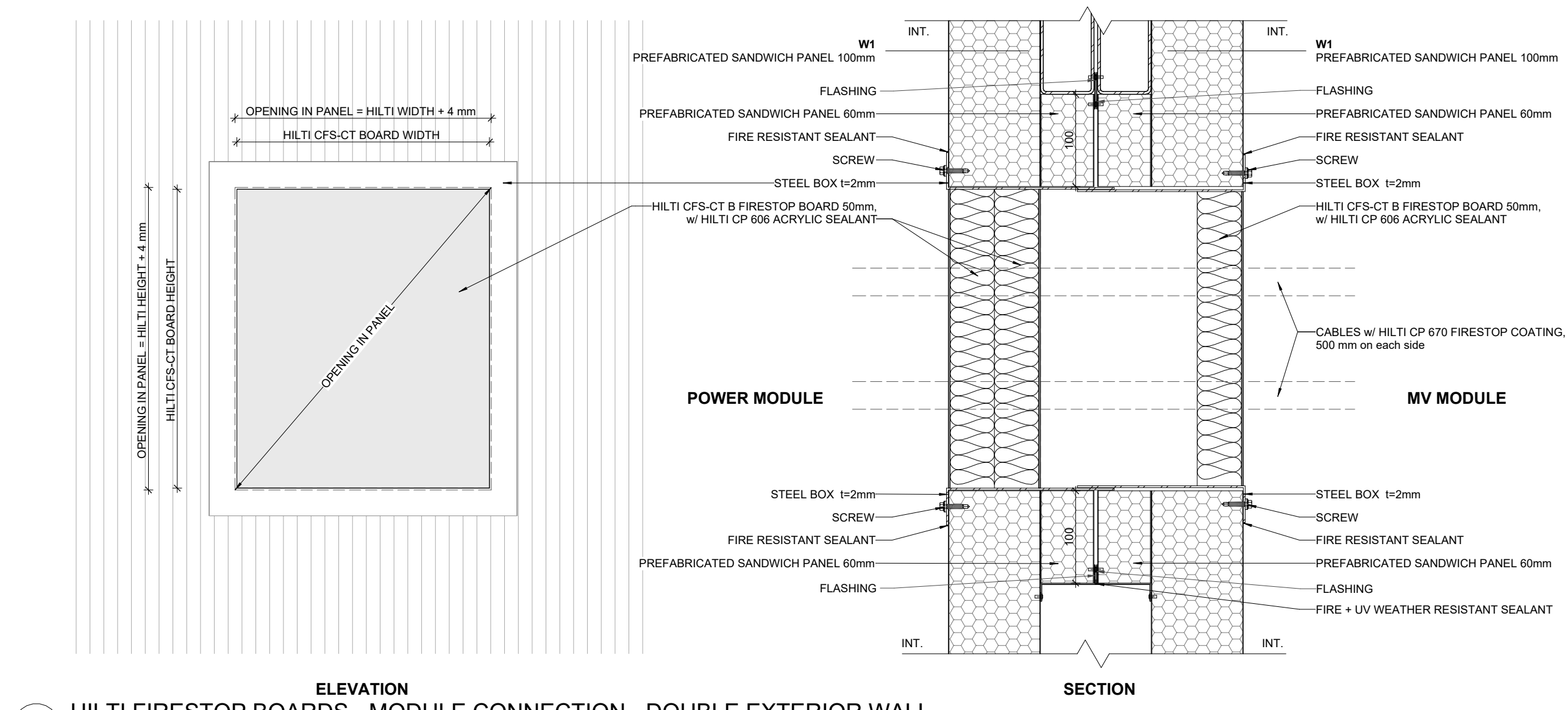
P04 HILTI FIRESTOP BOARDS - MODULE CONNECTION - DOUBLE EXTERIOR WALL 1:5
