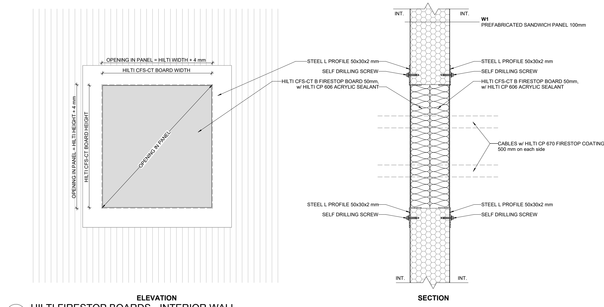
P05 HILTI FIRESTOP BOARDS - INTERIOR WALL 1:5
