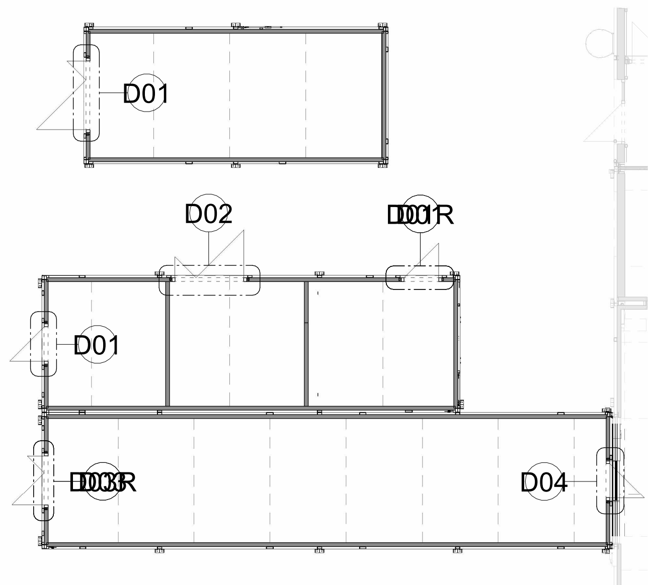
KEY PLAN - PM/MV/MS DOOR DETAIL POSITIONS
